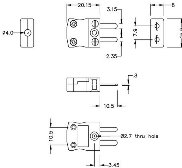
Miniature in-line Plug (dimensions in mm)
