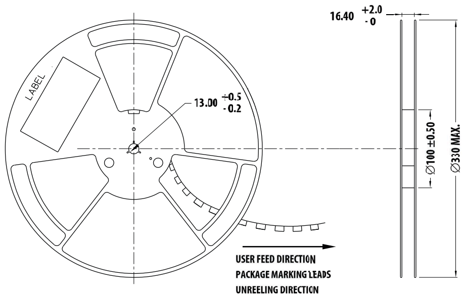
Figure 9: Reel Dimensions
