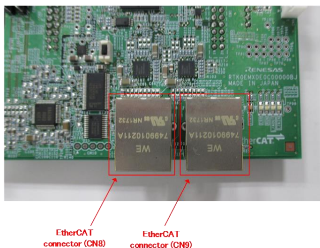
Figure 5-2 EtherCAT Connector
