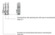
Example of a 2-pole terminal strip; with operating slot; with snap-in mounting feet
