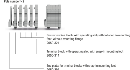
Example of a 5-pole terminal strip; with operating slot; with snap-in mounting feet
