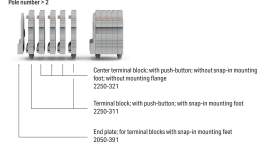
Example of a 5-pole terminal strip; with push-buttons; with snap-in mounting feet
