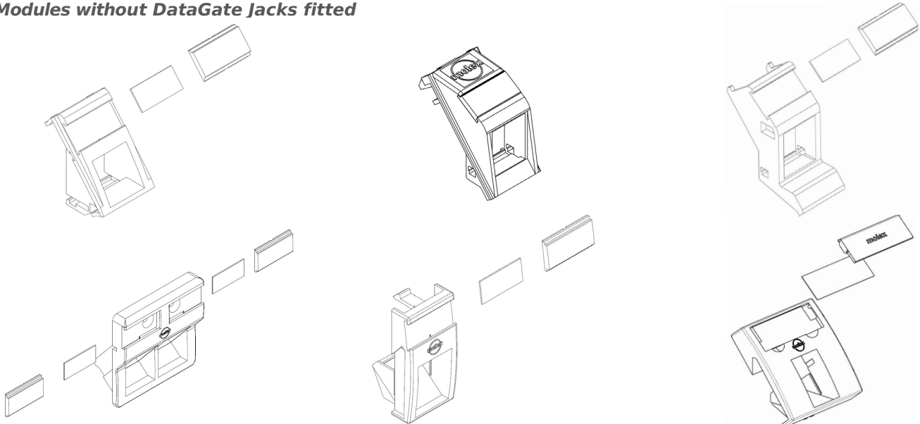
Top row, from left: MOD-Snap III module, Euromod II module, Contura module, Bottom row, from left: DIN module, 22.5 x 45mm module, 45 x 45mm module
