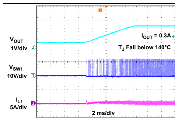
FIGURE 2-35: Thermal Shutdown Recovery.
