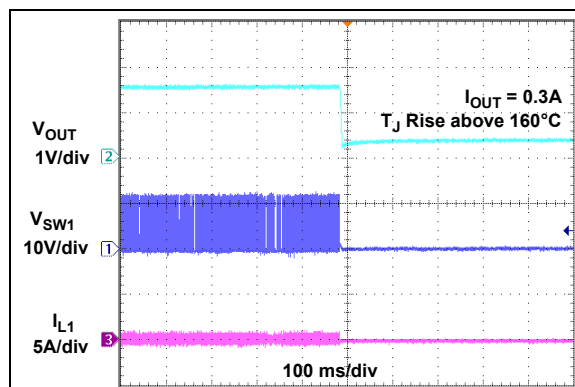
FIGURE 2-34: Thermal Shutdown.
