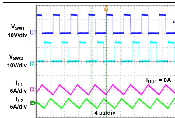
FIGURE 2-36: Switching Waveforms Phasing ( V_{OUT} = 5V , I_{OUT} = 0A ).
