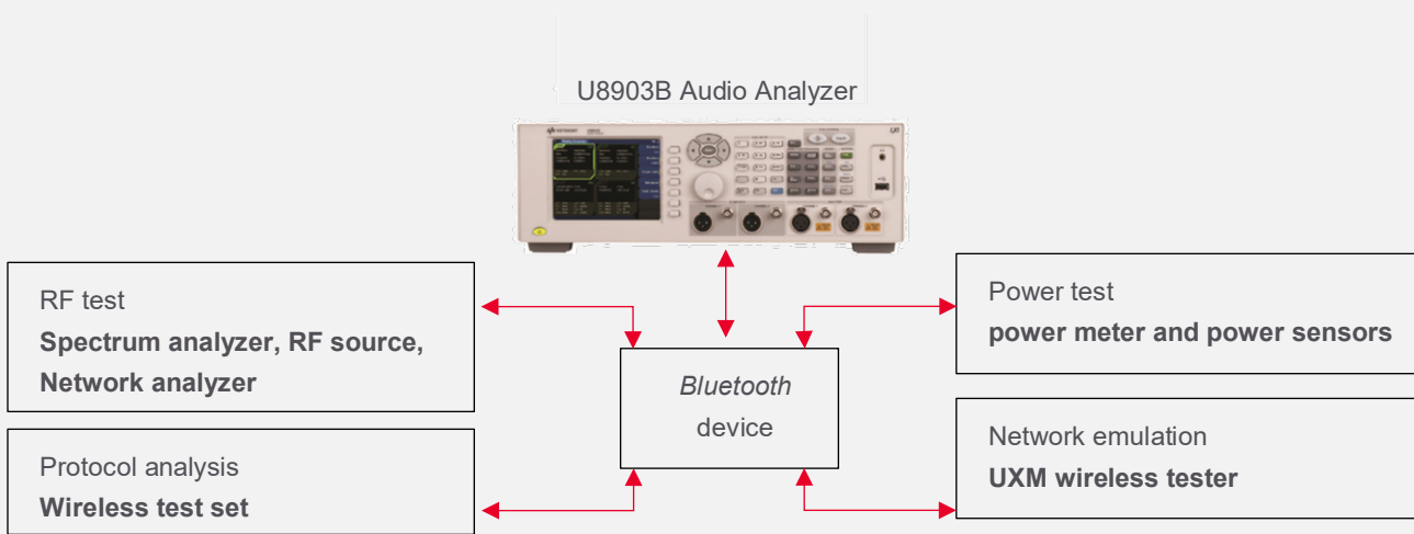
Figure 4. Total Keysight Bluetooth solution.
