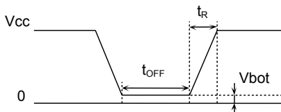
Figure 59. Rise waveform
