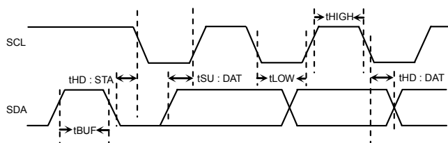
Figure 7. Serial Data Timing
