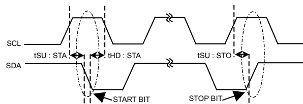
Figure 8. Start and Stop Bit Timing
