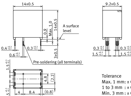
External dimensions
