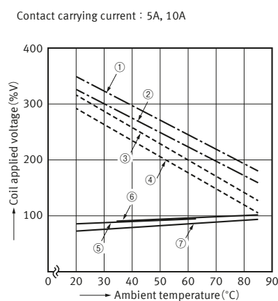
4-1. Ambient temperature characteristics (1 Form A)
