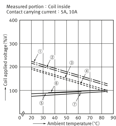
4-2. Ambient temperature characteristics (1 Form C)
