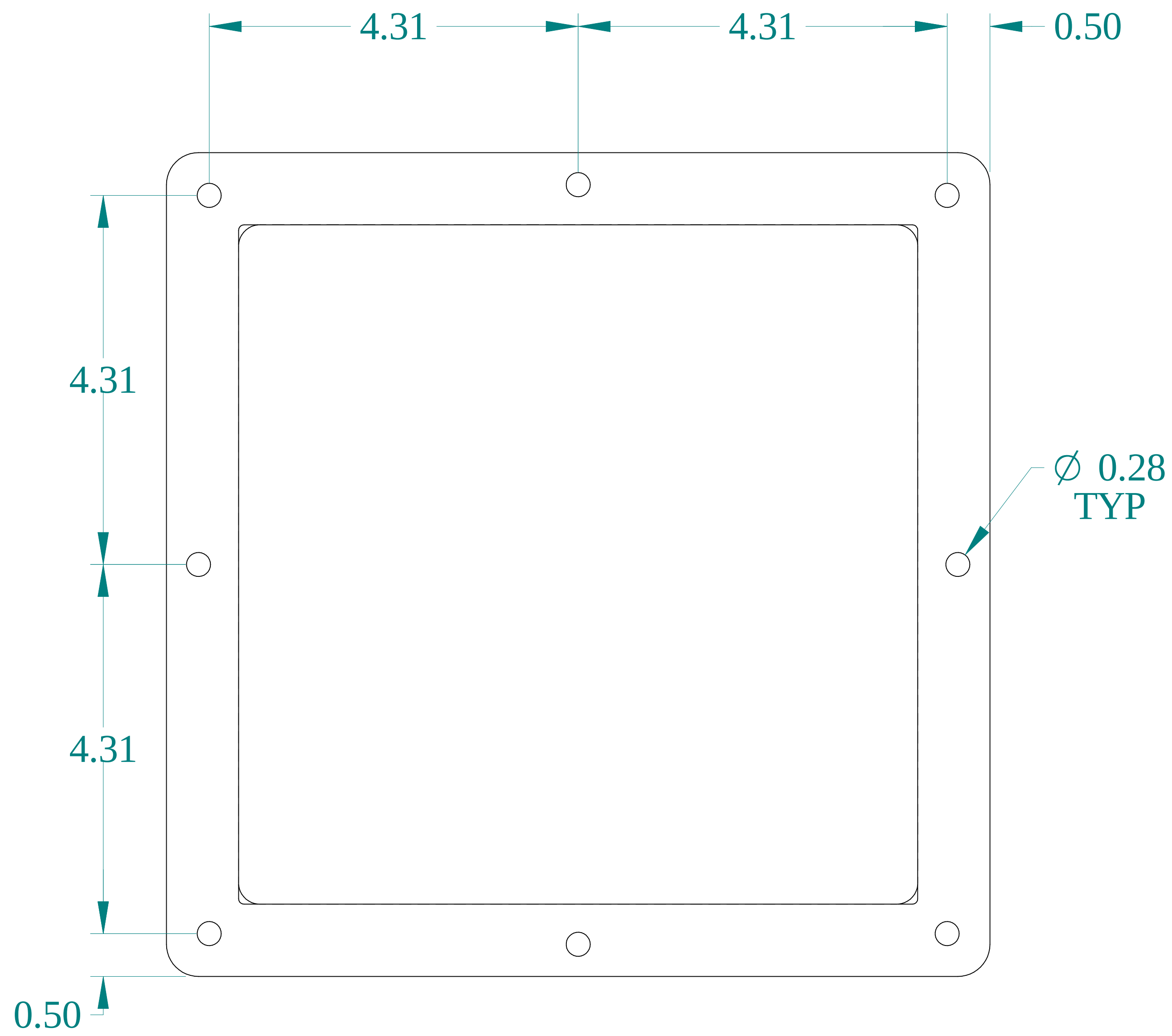
FRONT VIEW
