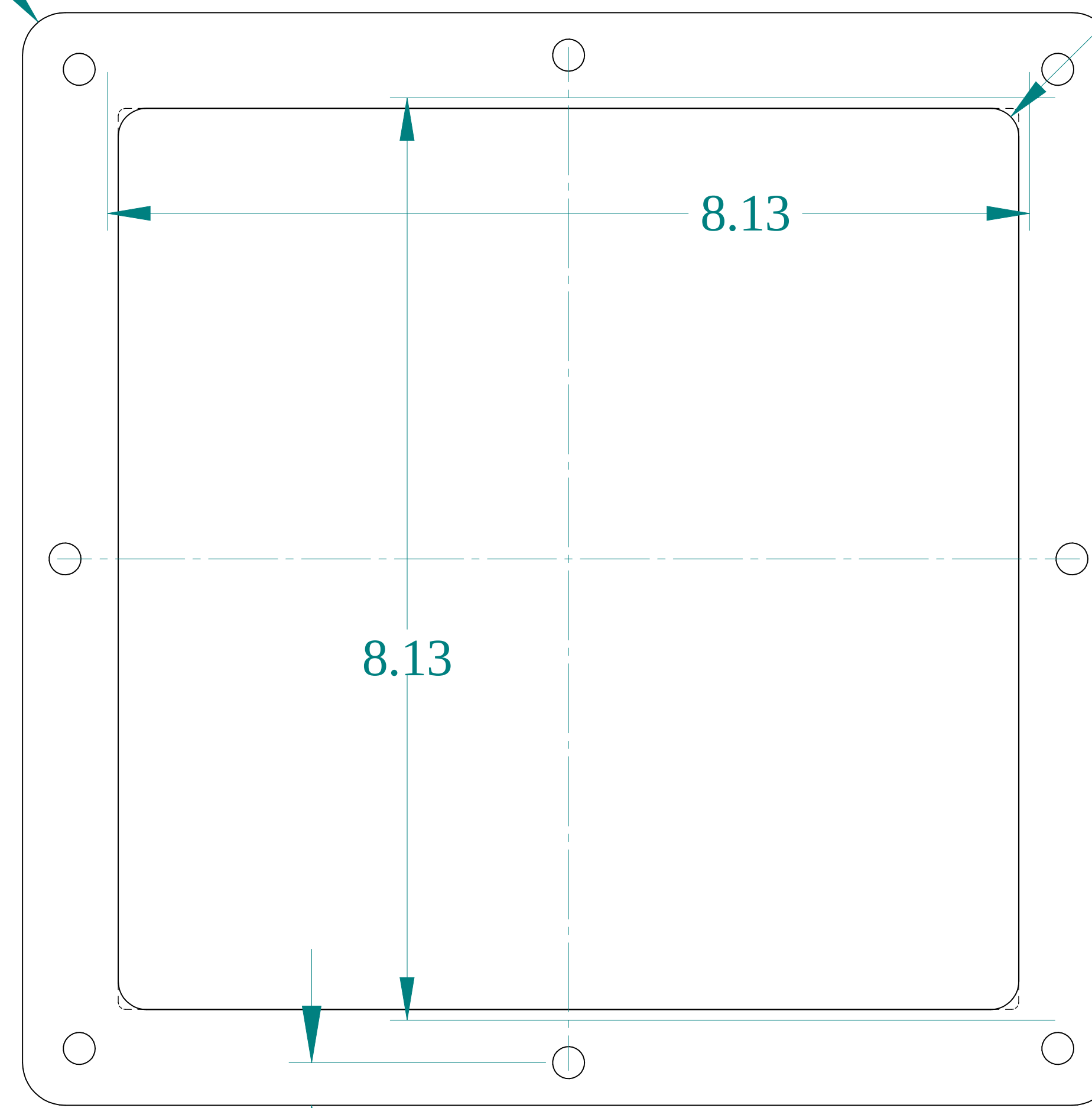
BACK VIEW
