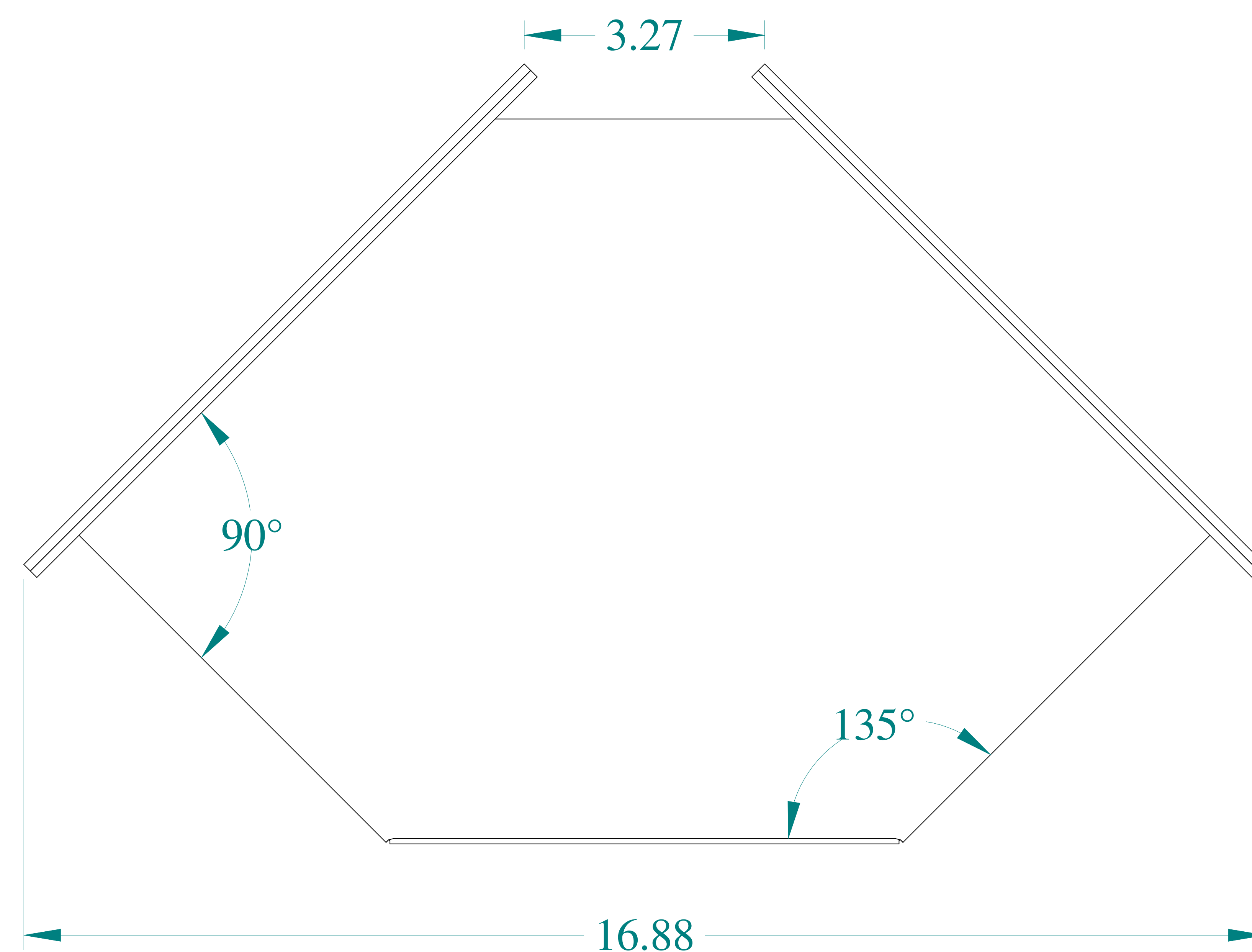
BOTTOM VIEW
