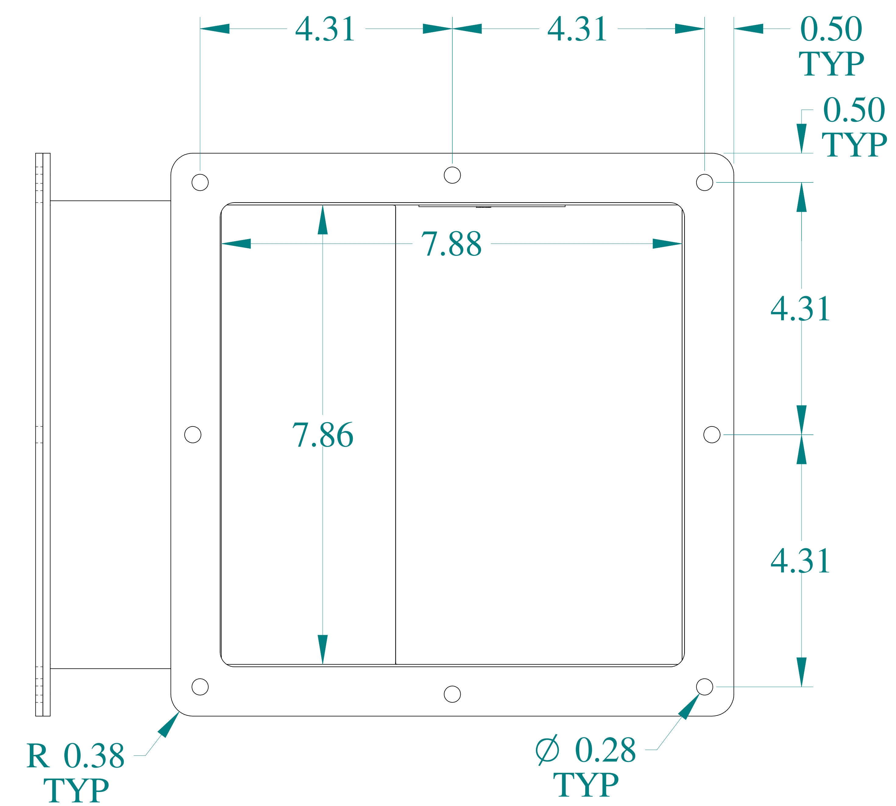
VIEW Z-Z
