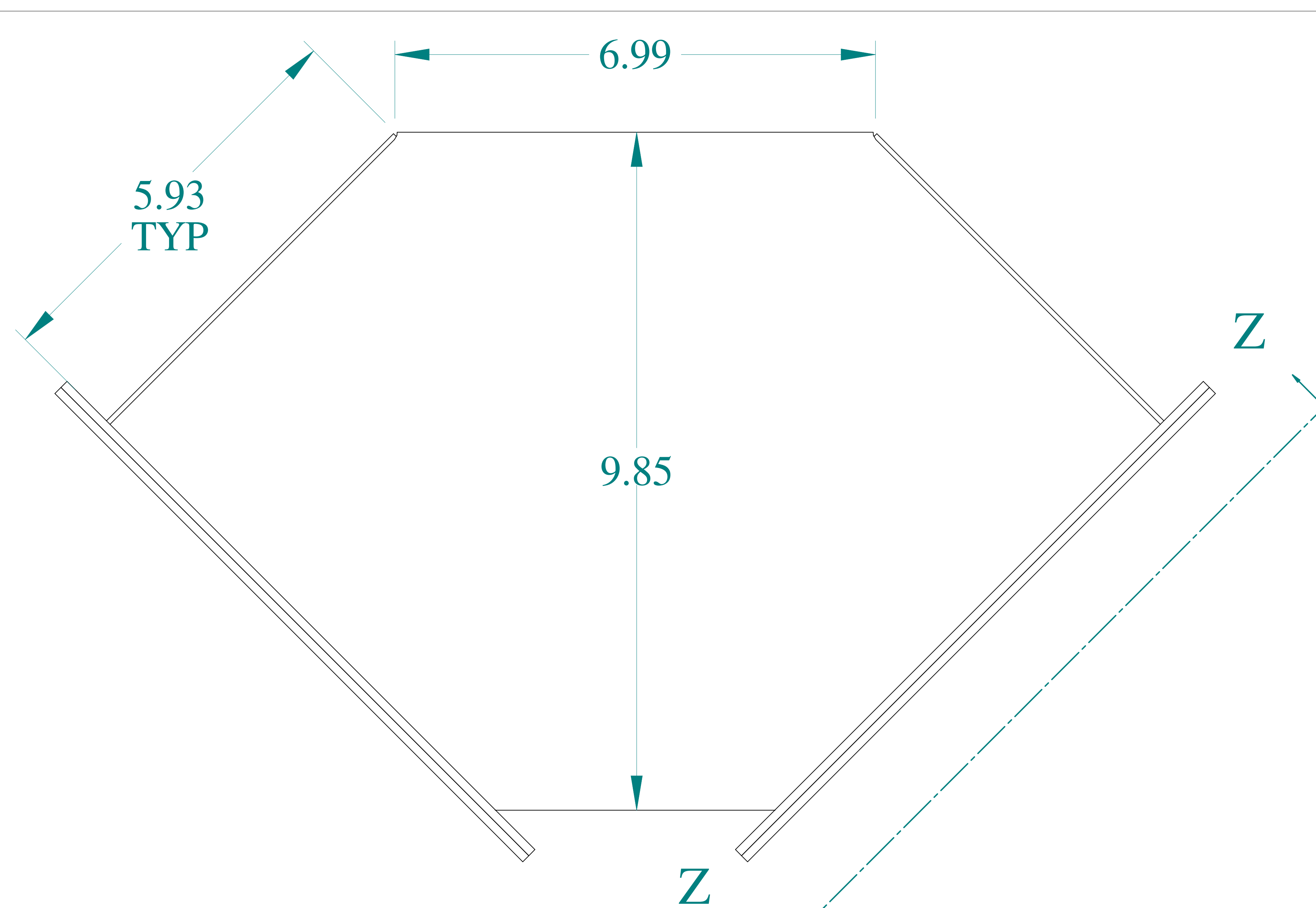
TOP VIEW
