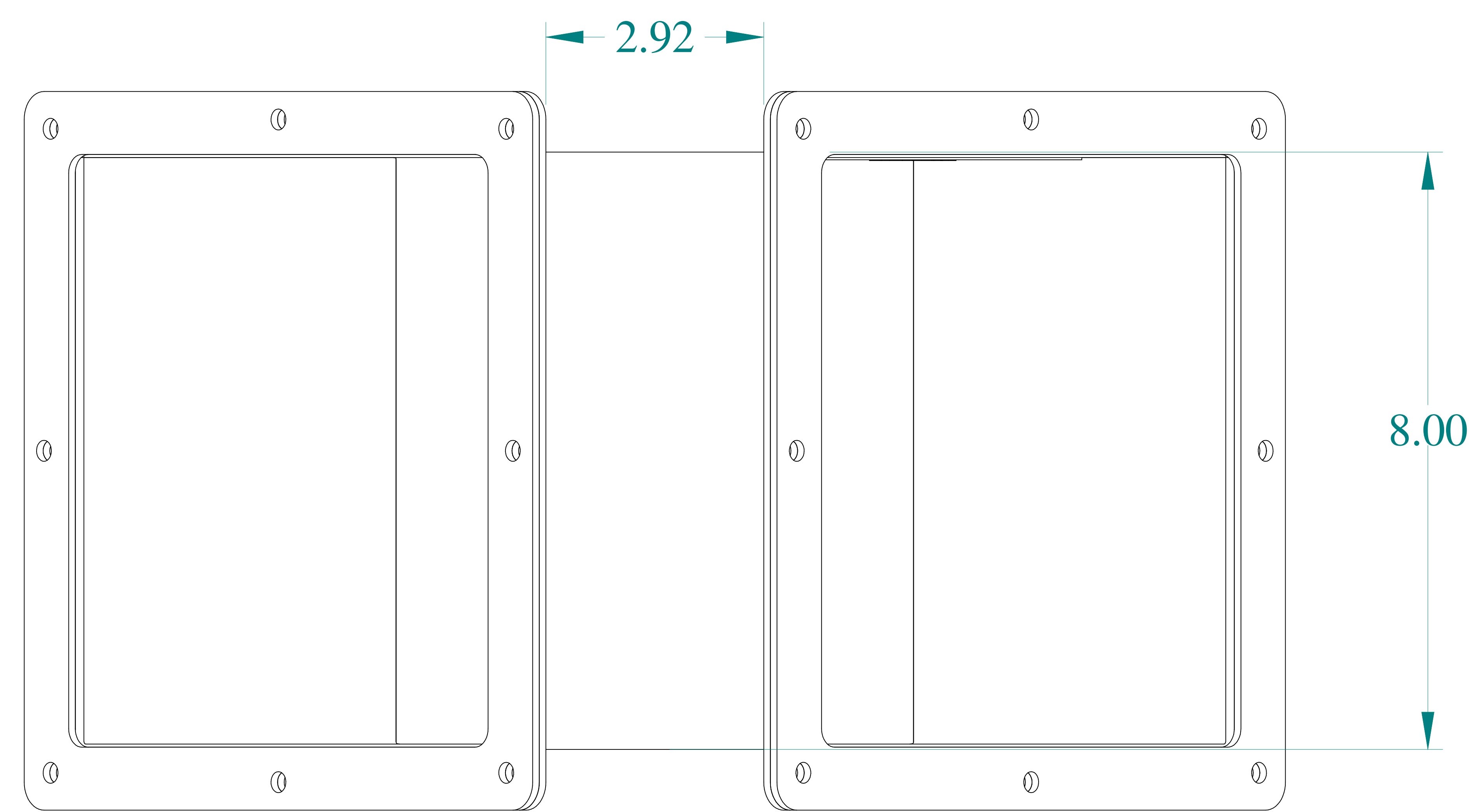
FRONT VIEW
