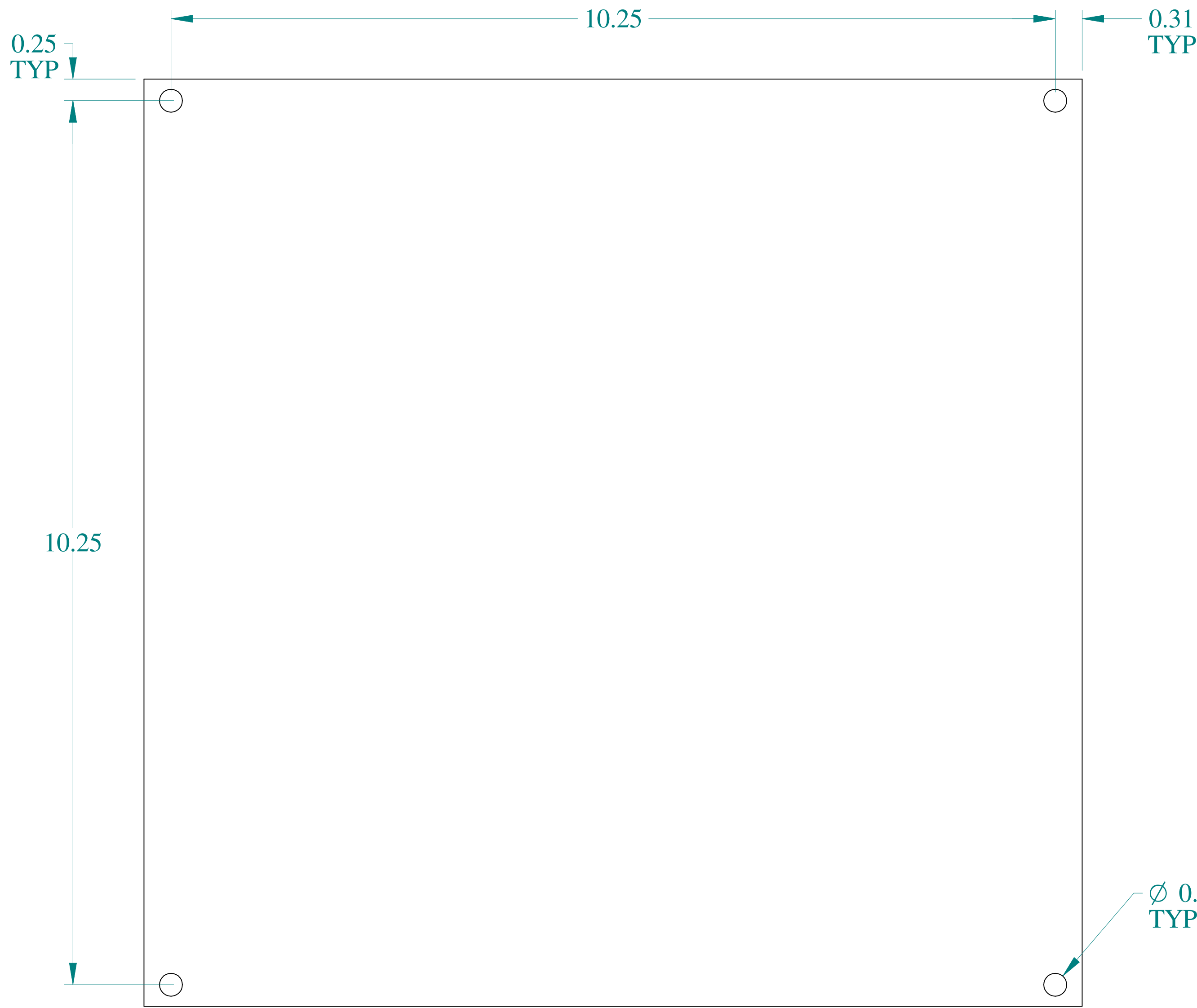
FRONT VIEW
