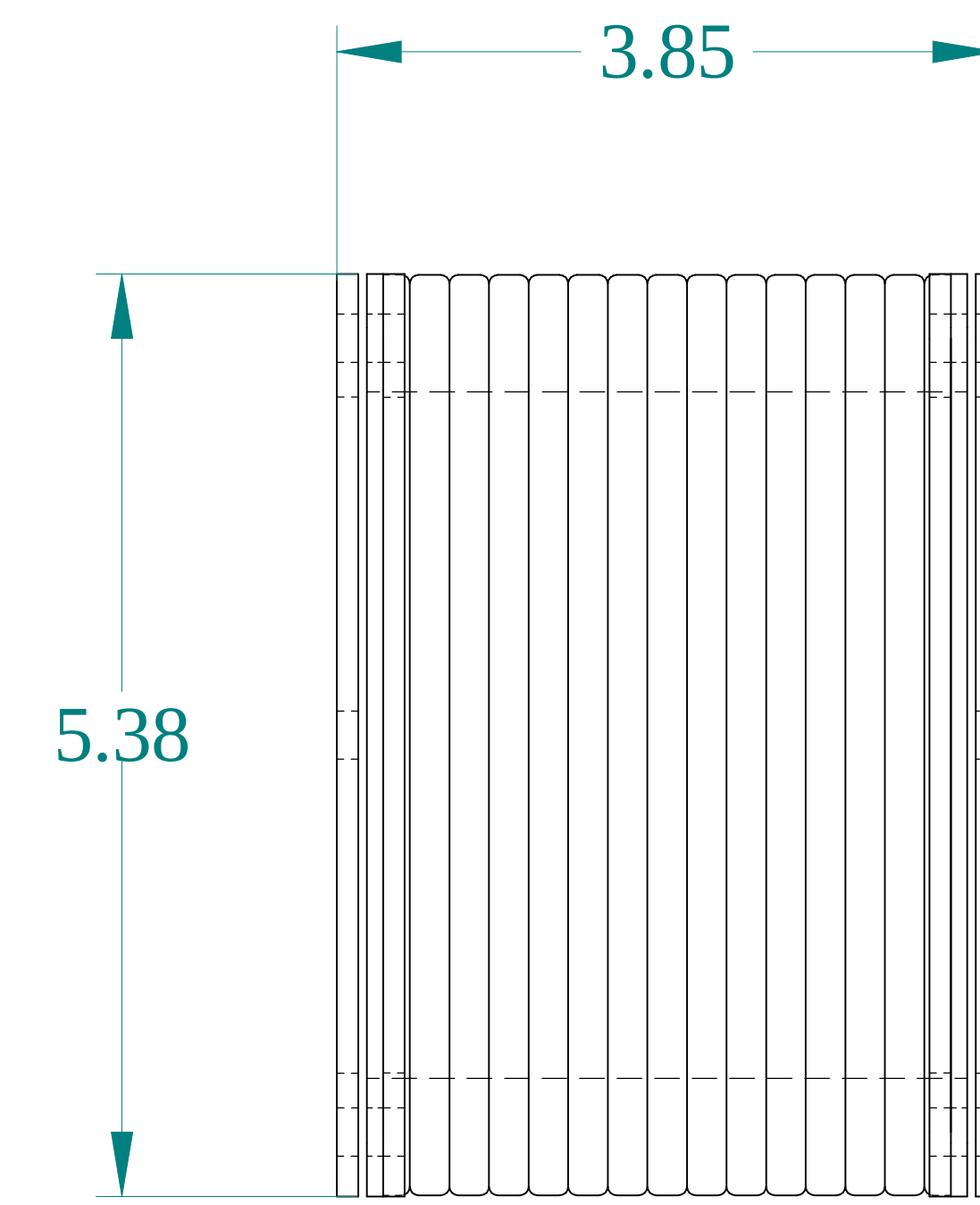
TOP VIEW
