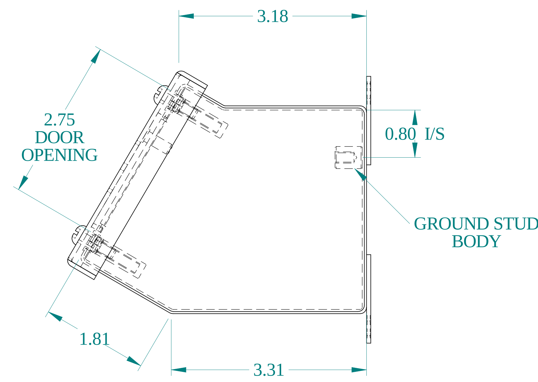
SIDE VIEW
