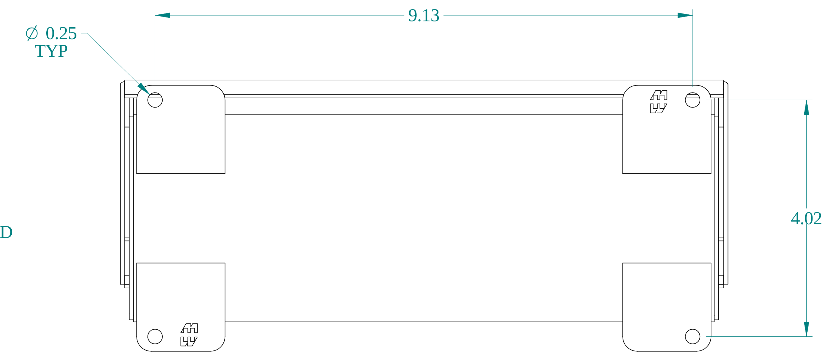
BACK VIEW
