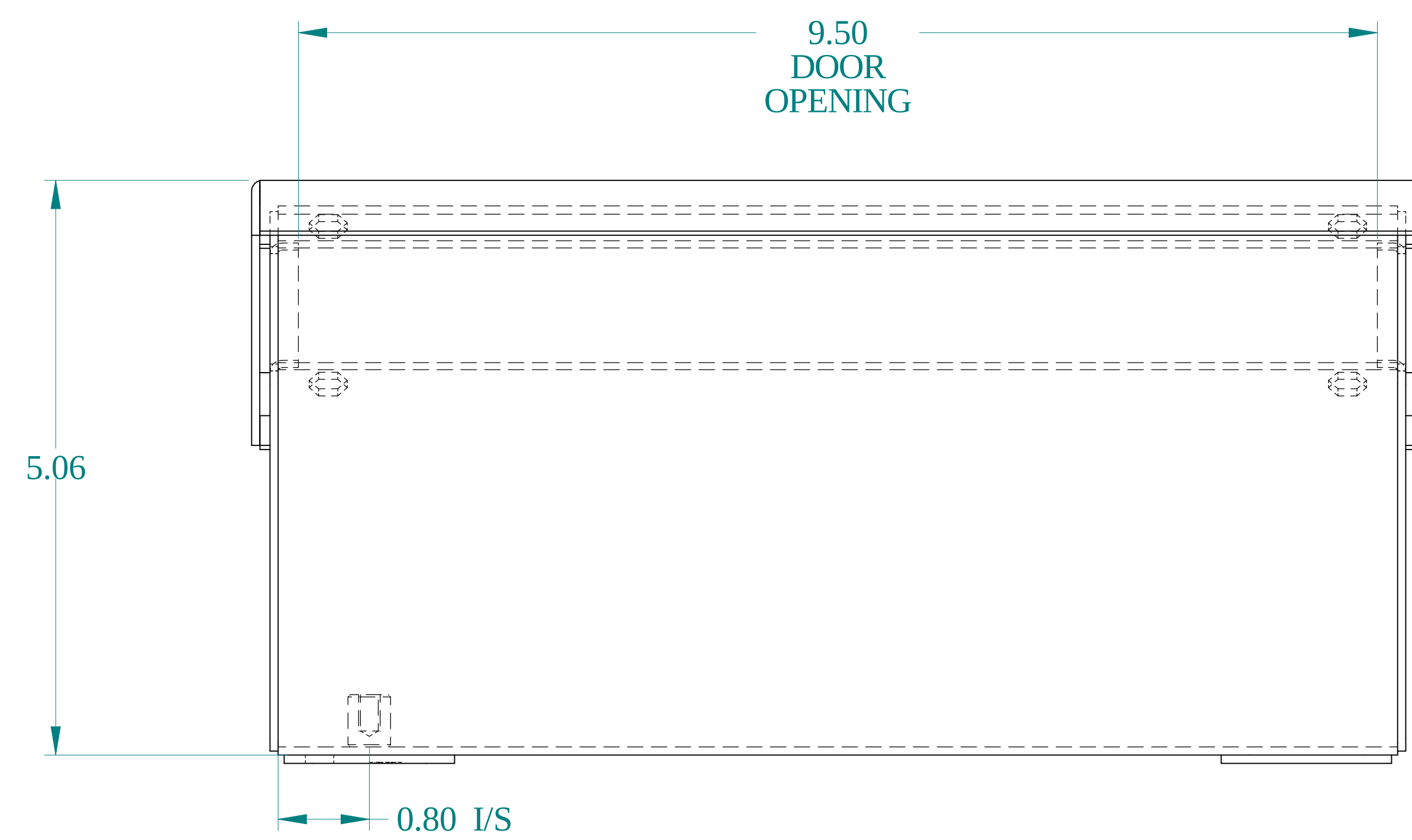
BOTTOM VIEW
