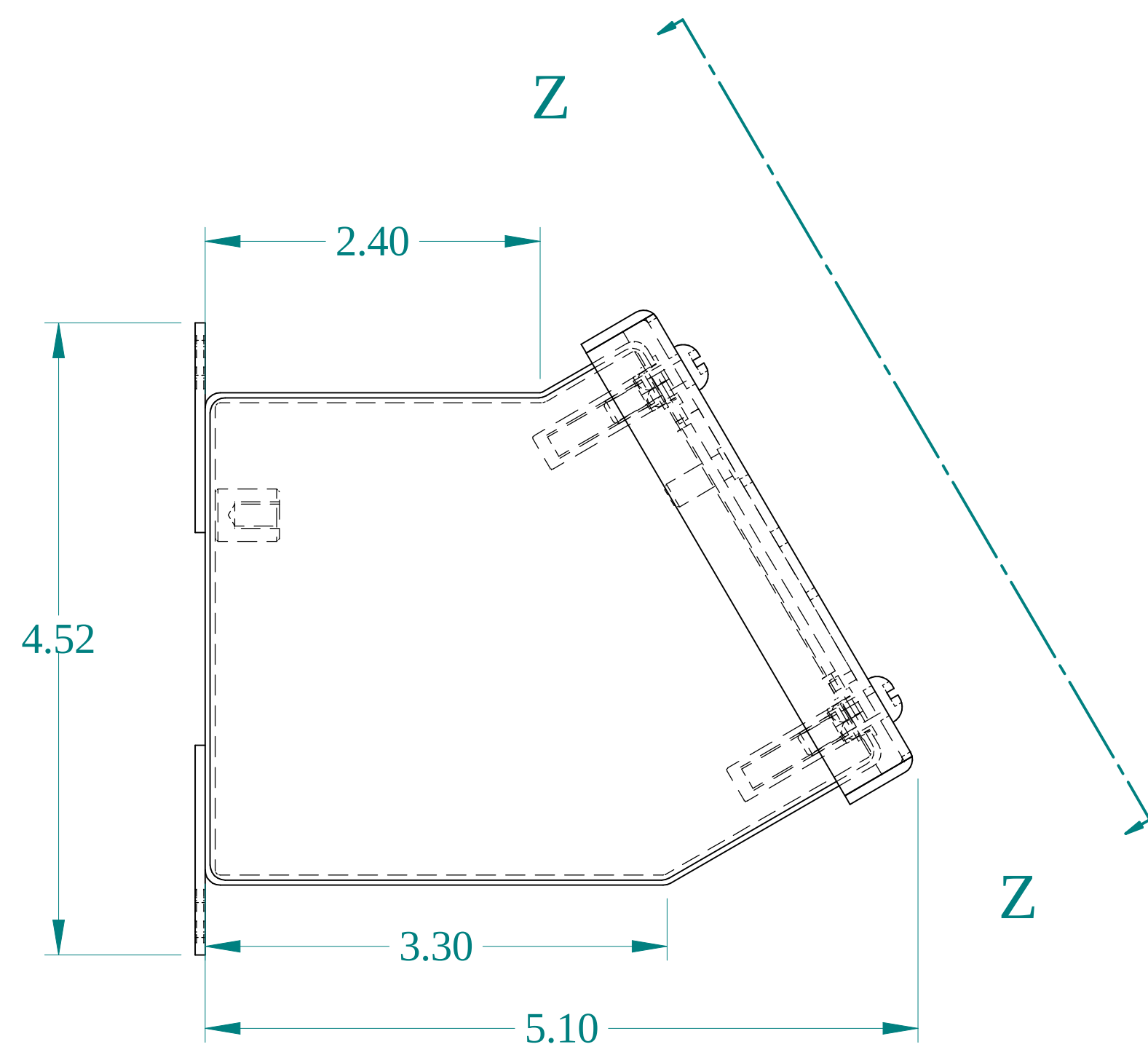
SIDE VIEW
