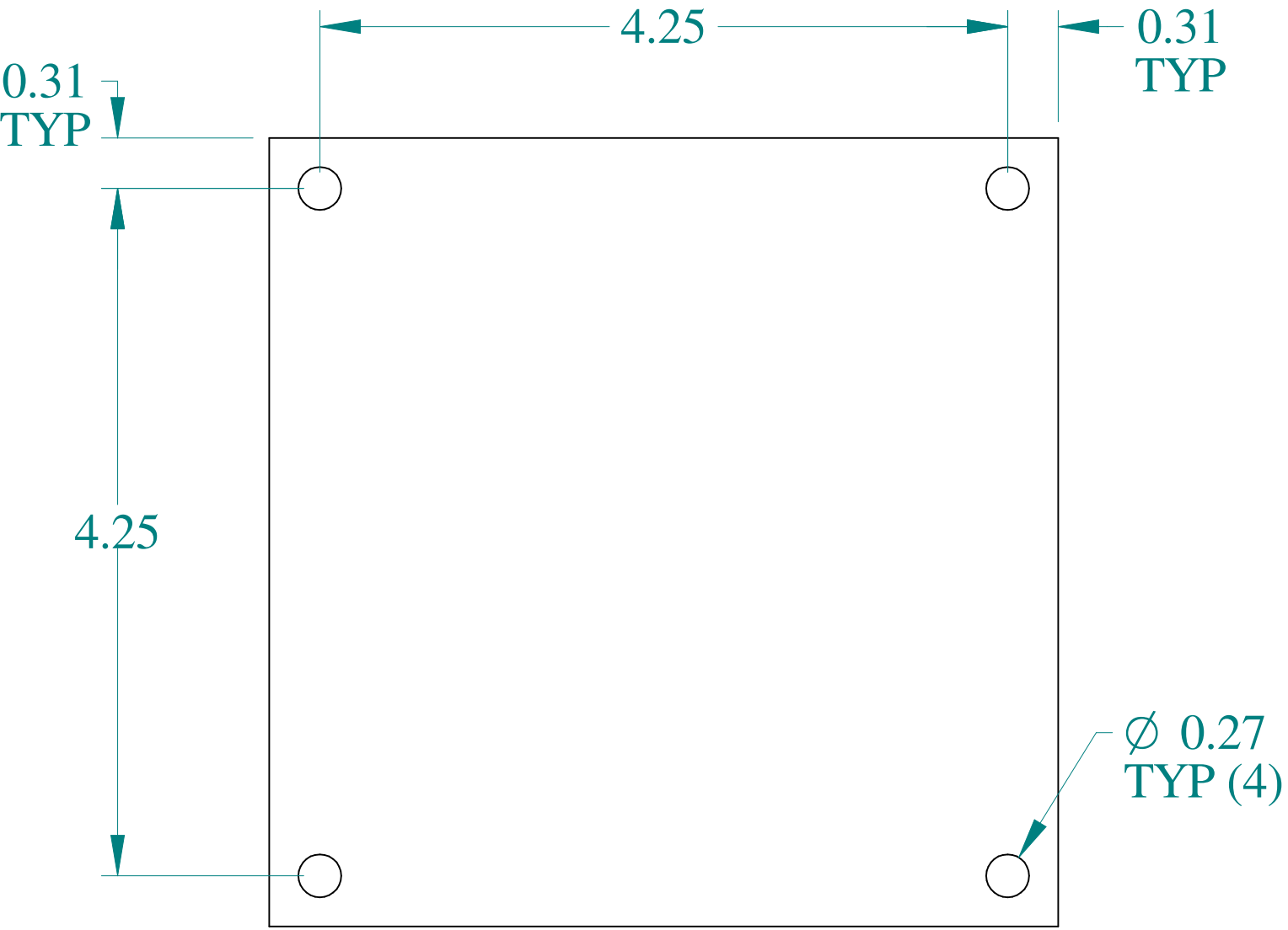
FRONT VIEW
