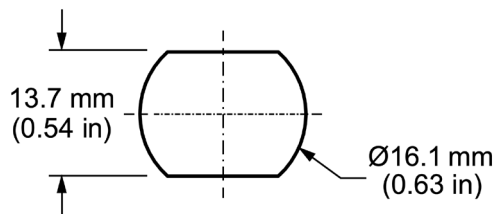
Figure 8. ANT-8/9-SPNF2 Mounting Hole Dimensions
