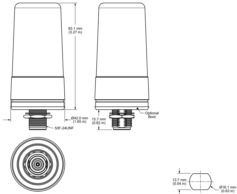
Figure 1. ANT-8/9-SPNF2 Dimensions
