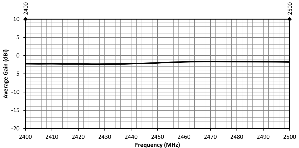
Figure 8. ANT-2.4-WRT Antenna Average Gain, Free Space
