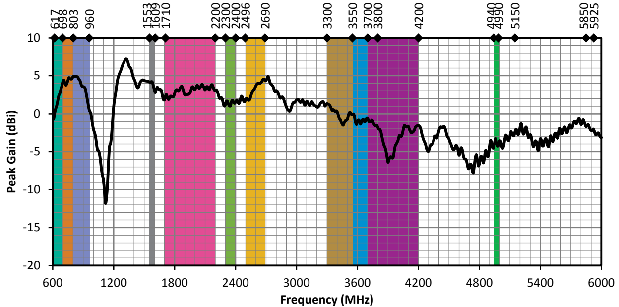
Figure 4. ANT-LTE-VDP-2000-SMA Peak Gain with Frequency Band Highlights
