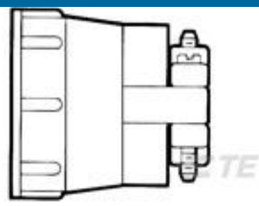
TE Part #207774-3 CLAMP CABLE SHELL, SIZE 23
