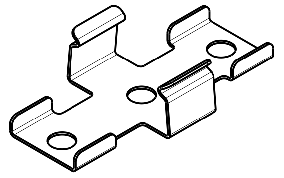
ISOMETRIC VIEW SCALE 3:2
