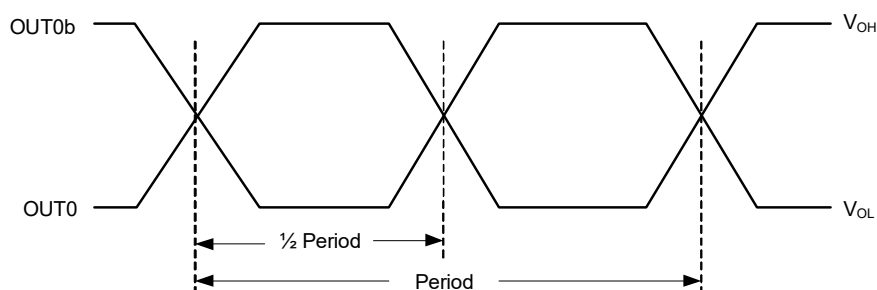
Figure 4. Differential Waveform Measurement Points
