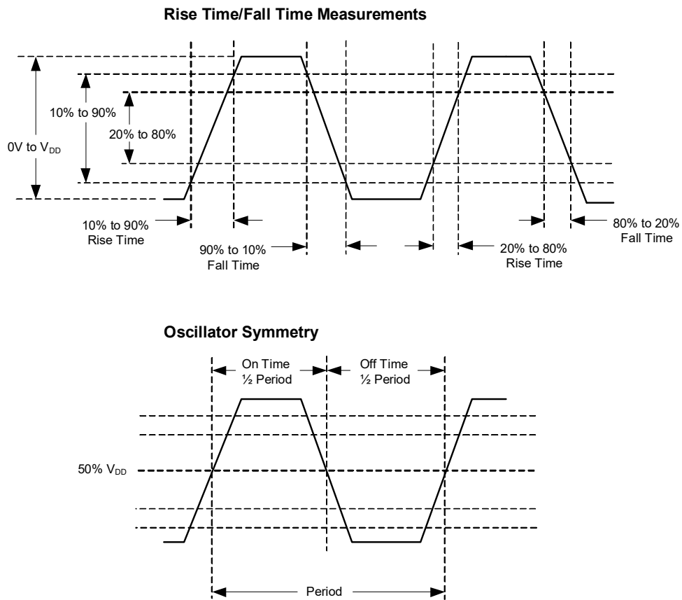
Figure 5. LVCMOS Waveform Measurement Points
