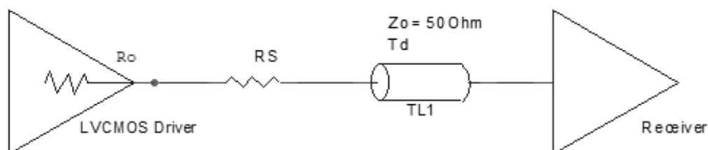
Figure 16. LVCMOS Output Termination
