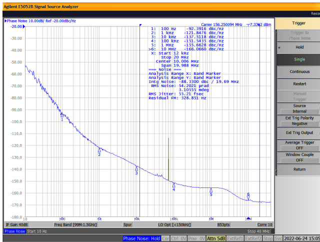
Figure 6. 1.8V LVCMOS, 156.25MHz
