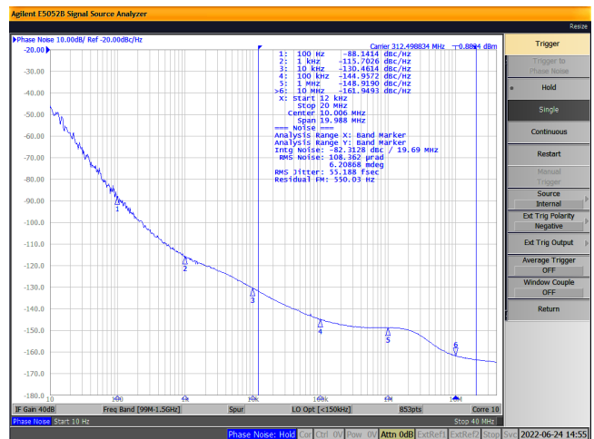
Figure 9. 3.3V LVPECL, 312.5MHz
