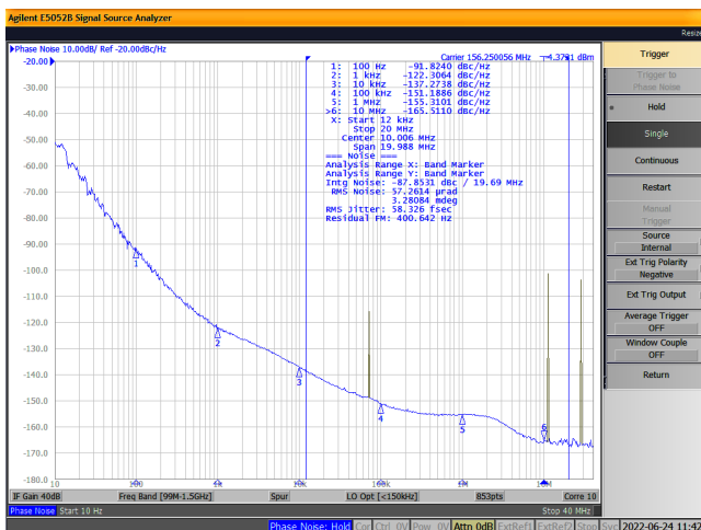
Figure 10. 1.8V HCSL, 156.25MHz
