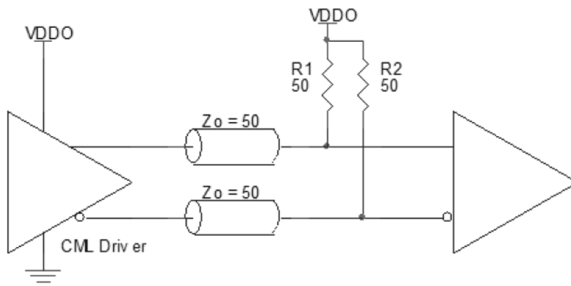
Figure 12. CML Output Termination
