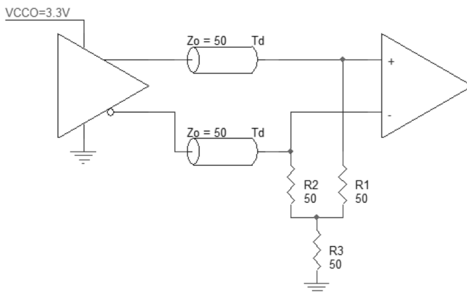
Figure 13. 3.3V LVPECL Output Termination
