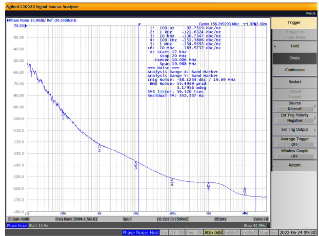
Figure 7. 3.3V HCSL, 156.25MHz
