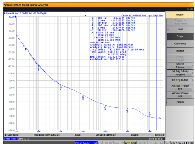
Figure 11. 3.3V CML, 312.5MHz
