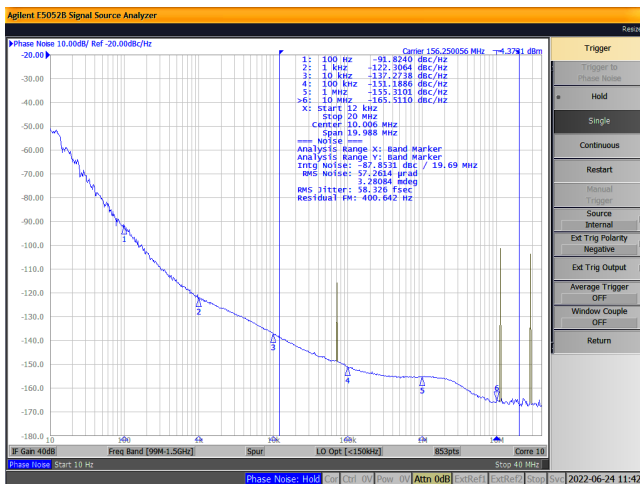
Figure 8. 1.8V LVDS, 156.25MHz
