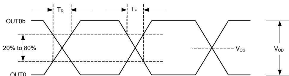
Output Levels/Rise Time/Fall Time Measurements
