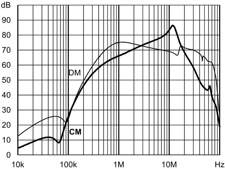
Attenuation graph
