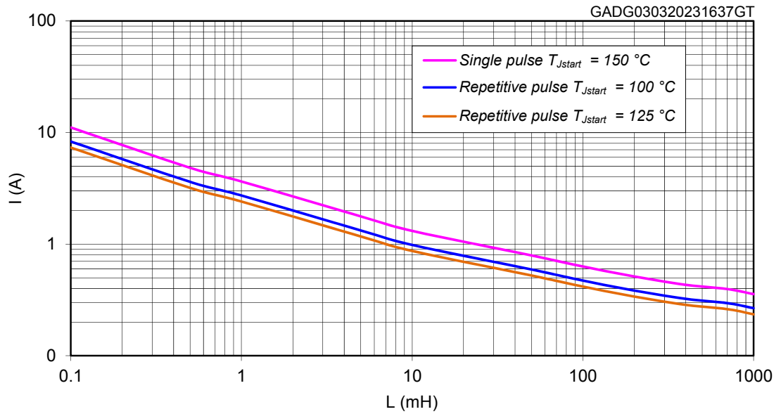
Figure 39. Maximum turn off current versus inductance
