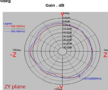
Phi=90.00deg
