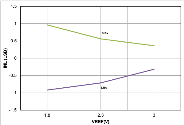
Figure 41-7. ADC, Single-Ended INL, V_{DD} = 3.0V , T_{AD} = 1\mu S
