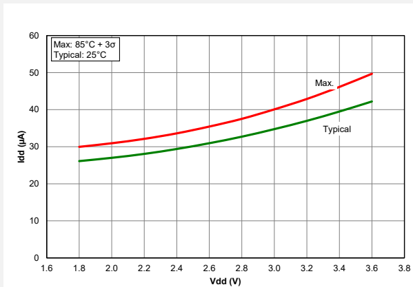
Figure 41-63. I_{DD} , Fixed Voltage Reference (FVR), PIC18LF65/66K40 only
