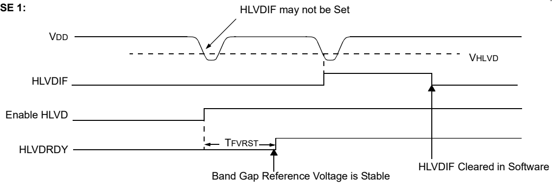
Figure 35-2. Low-Voltage Detect Operation (INTL = 1)
