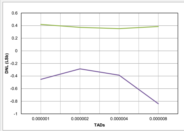
Figure 41-6. ADC, Single-Ended DNL, V_{DD} = 3.0V , V_{REF} = 3.0V
