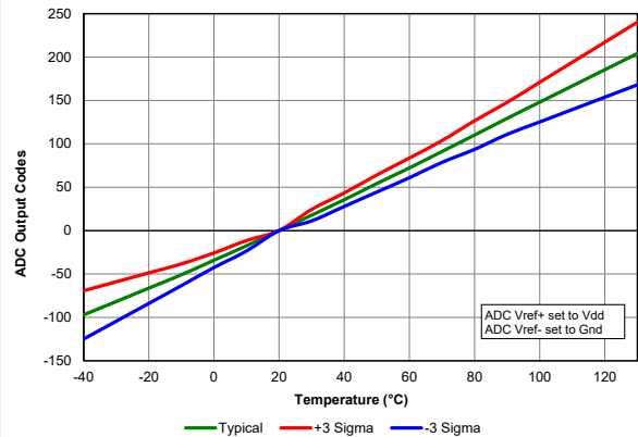
Figure 41-90. Temperature Indicator, Slope Normalized to 20°C, High Range, V_{DD} = 3.0V
