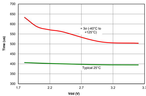
Figure 41-105. Wake From Sleep, LFINTOSC, PIC18LF65/66K40 only
