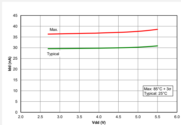
Figure 41-64. I_{DD} , Fixed Voltage Reference (FVR), PIC18F65/66K40 only
