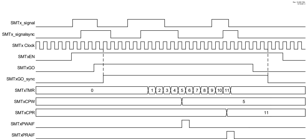
Figure 26-6. Period and Duty Cycle, Single Acquisition Mode Timing Diagram
