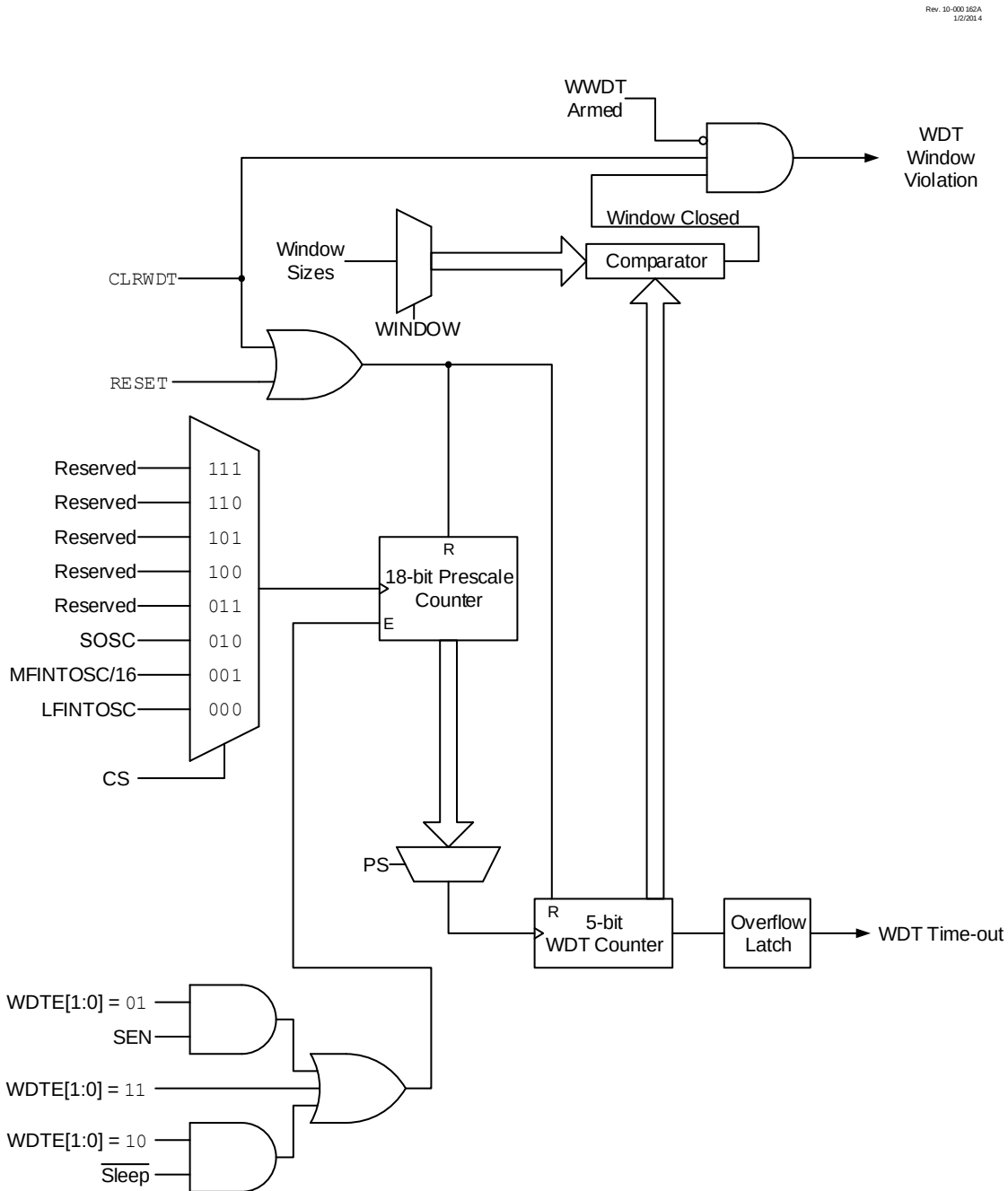
Figure 9-1. Windowed Watchdog Timer Block Diagram
