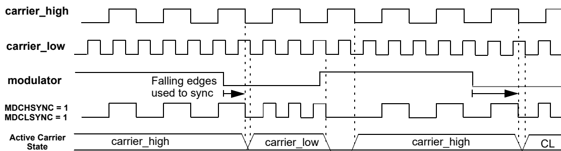
Figure 27-6. Full Synchronization (MDCHSYNC = 1, MDCLSYNC = 1)
