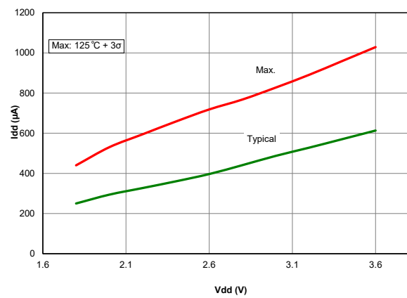
Figure 41-50. I_{DD} , ECM Oscillator, F OSC = 4MHz, PIC18LF65/66K40 only
