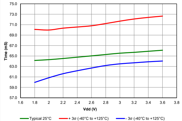
Figure 41-84. Power-up Timer Period, PIC18LF65/66K40 only
