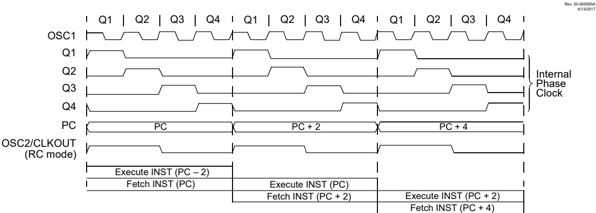
Figure 10-4. Clock/Instruction Cycle
