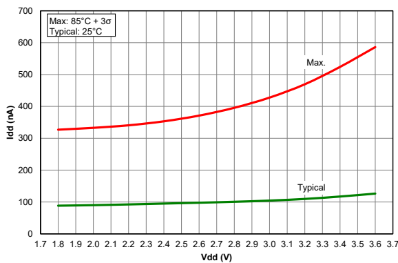
Figure 41-69. I_{PD} , Comparator, PIC18LF65/66K40 only
