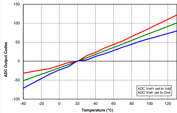
Figure 41-92. Temperature Indicator, Slope Normalized to 20°C, Low Range, V_{DD} = 3.0V
