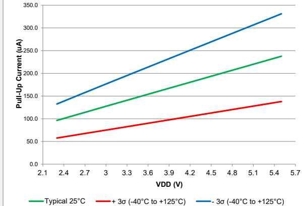
Figure 41-108. Weak Pull-up Current, PIC18F65/66K40 only
