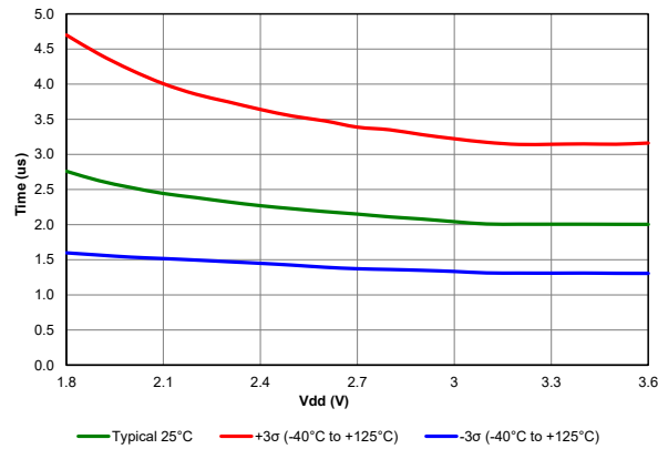
Figure 41-9. ADC RC Oscillator Period, PIC18LF65/66K40 only
