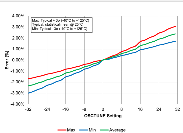
Figure 41-78. OSCTUNE Center Frequency
