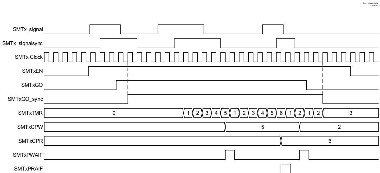
Figure 26-7. High and Low Measurement Mode, Repeat Acquisition Timing Diagram
