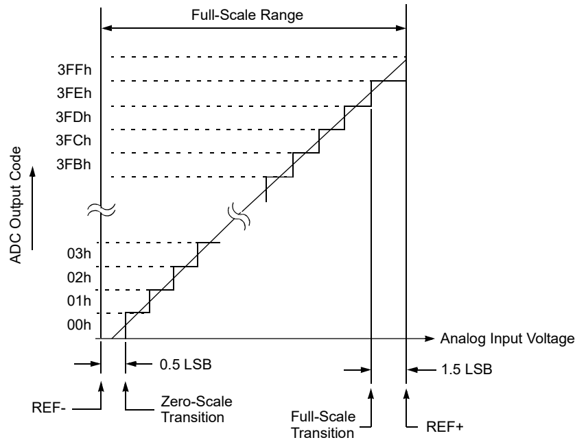
Figure 33-5. ADC Transfer Function
