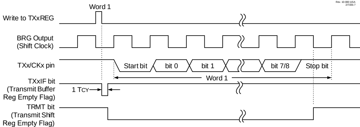
Figure 29-3. Asynchronous Transmission
