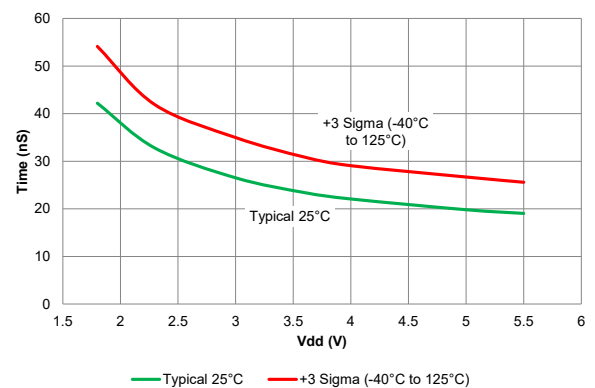
Figure 41-58. I/O Fall Time, Slew Rate Control Enabled
