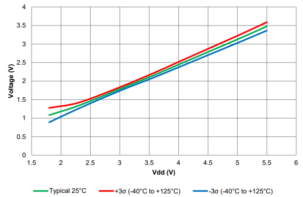
Figure 41-54. Schmitt Trigger High Values
