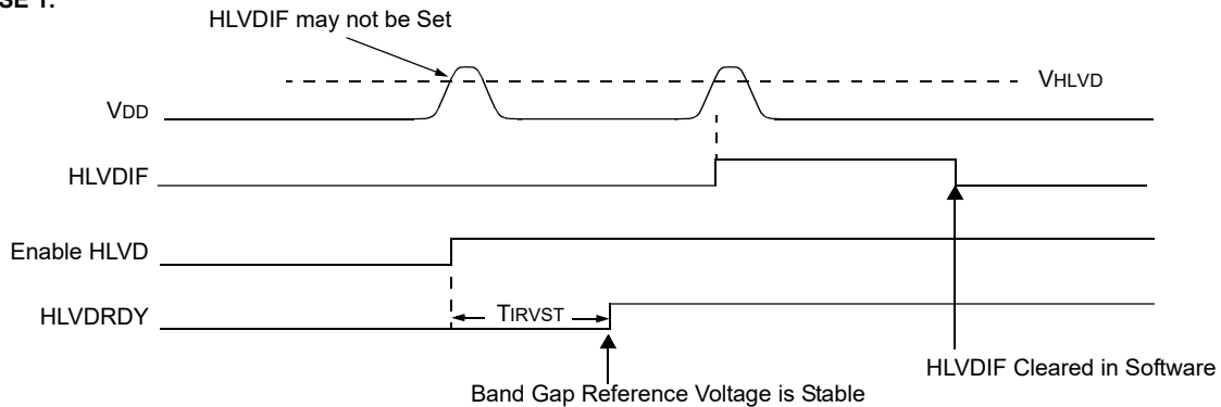
Figure 35-3. High-Voltage Detect Operation (INTH = 1)
