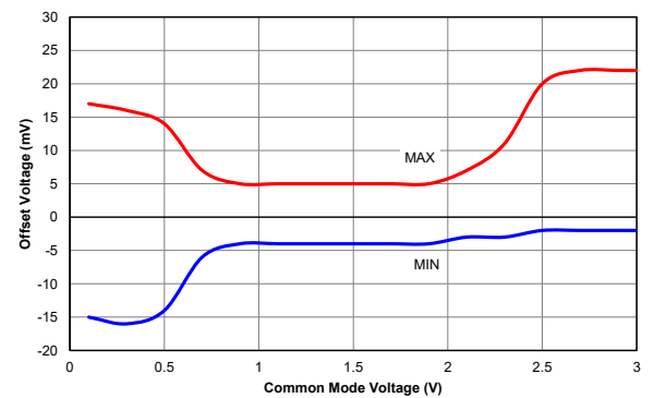
Figure 41-28. Comparator Offset, V DD = 3.0V, from -40°C to 125°C
