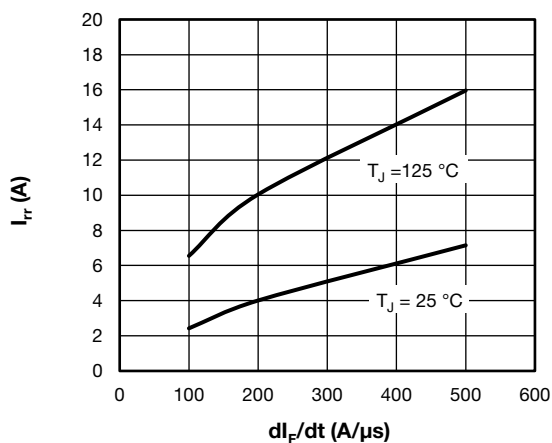
Fig. 15 - Typical Diode Reverse Recovery Current vs. dI_F/dt I_F = 50 A, V_{CC} = 400 V
