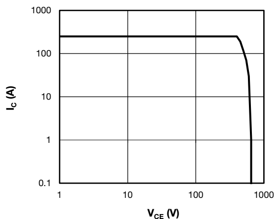
Fig. 17 - Trench IGBT Reverse BIAS SOA T_J = 175^\circ\text{C} , I_C = 250\text{ A} , R_g = 10\ \Omega , V_{GE} = +15\text{ V/0 V} , V_{CC} = 400\text{ V} , V_p = 650\text{ V}
