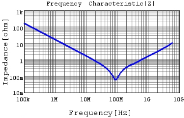
GRM155R71H103KA88 |Z| DC0V, 25degC
