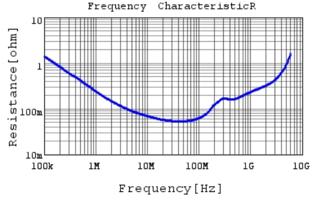
GRM155R71H103KA88 R DC0V, 25degC
