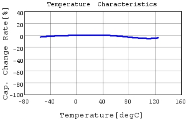
GRM155R71H103KA88 C-Temp. capchange, DC0.0V,
