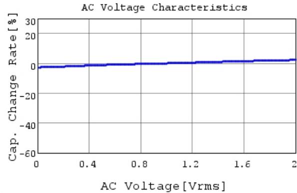
GRM155R71H103KA88 C-AC Voltage capchange, DC
