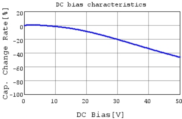
GRM155R71H103KA88 C-DC bias capchange, 25.0c
