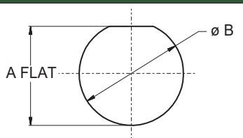
Jam-Nut Panel Cutout
