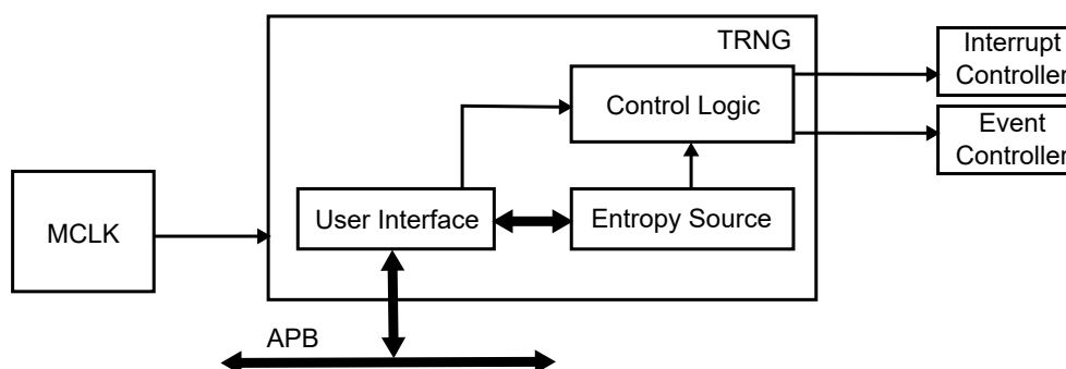
Figure 37-1. TRNG Block Diagram.
