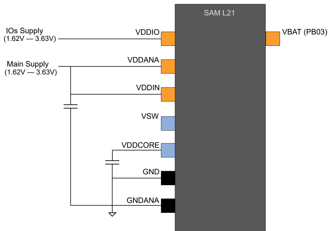
Figure 9-1. Power Supply Connection for Linear Mode Only
