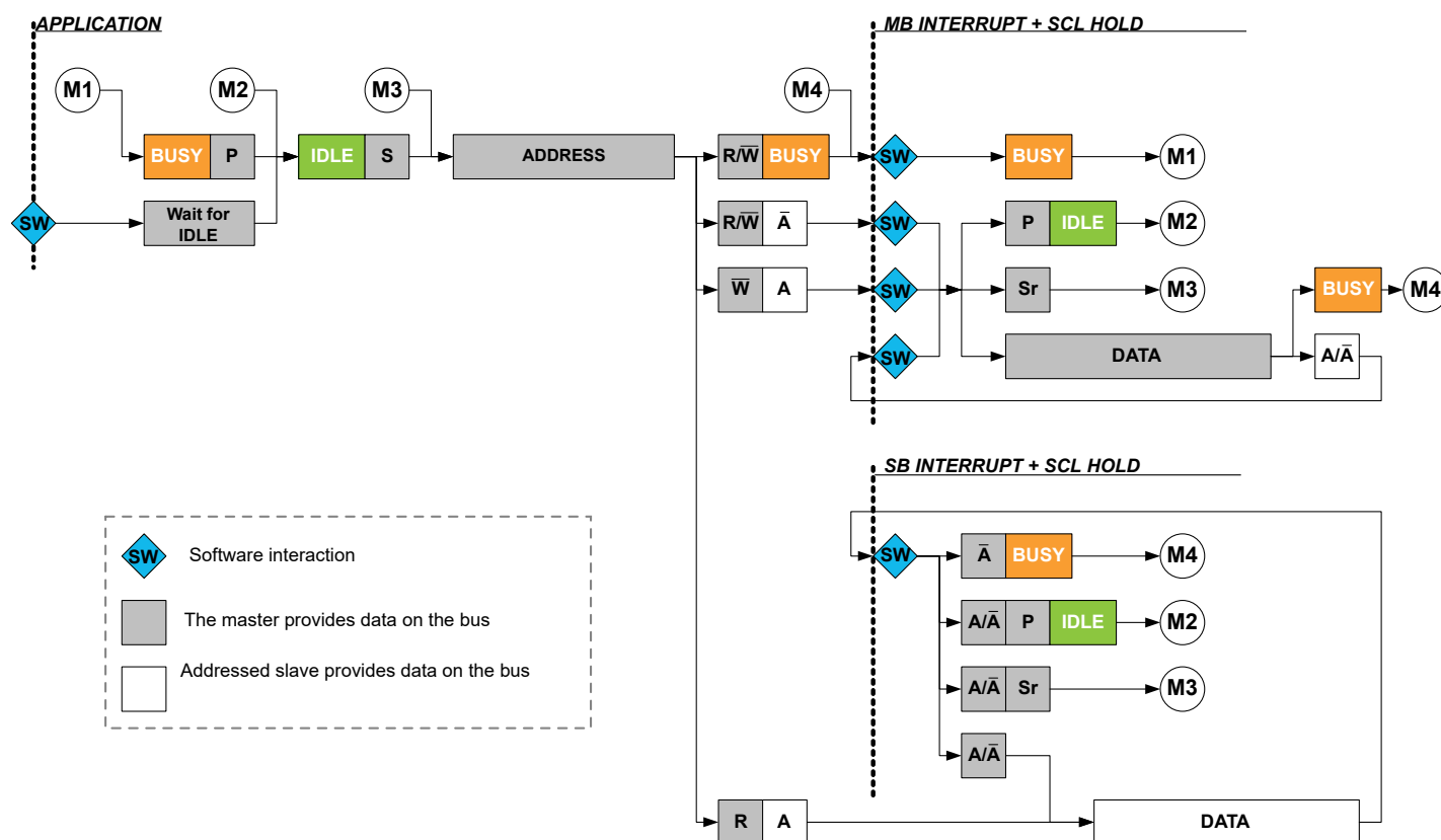
Figure 34-4. I 2 C Host Behavioral Diagram (SCLSM=0)
