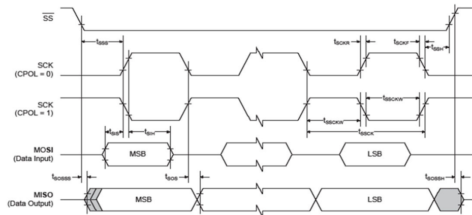
Figure 46-8. SPI Timing Requirements in Client Mode
