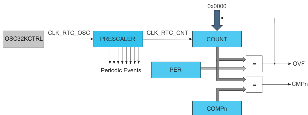
Figure 25-2. RTC Block Diagram (Mode 1 — 16-Bit Counter)
