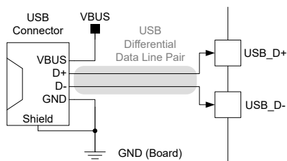
Figure 51-15. Low Cost USB Interface Example Schematic
