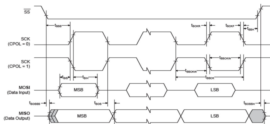
Figure 46-6. SPI Timing Requirements in Client Mode
