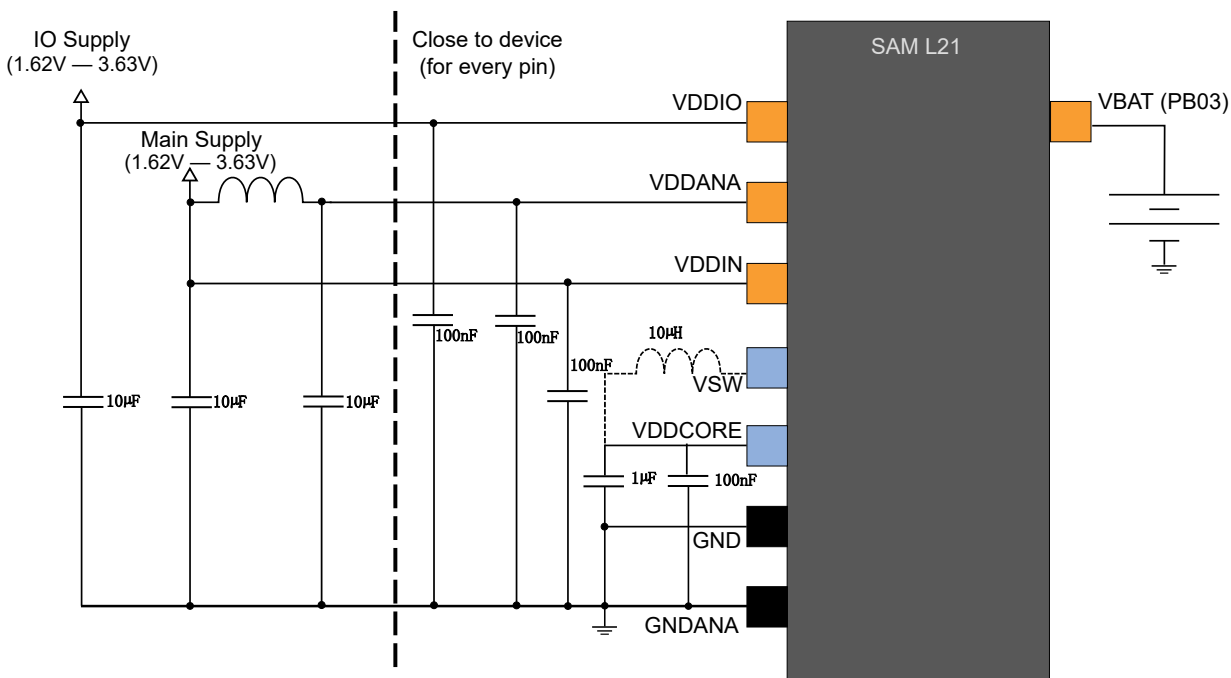
Figure 51-3. Power Supply Connection for Battery Backup
