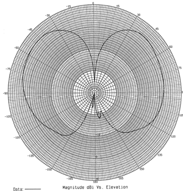
PSTGO 2400HS – Elevation Plot
