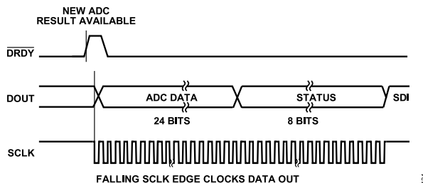
Figure 130. \overline{PIN} Mode Data Output Format (Without the \overline{CS} Signal)
