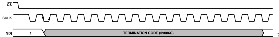
Figure 148. Exiting the Continuous Read Mode ( \overline{CS} = 0 )
