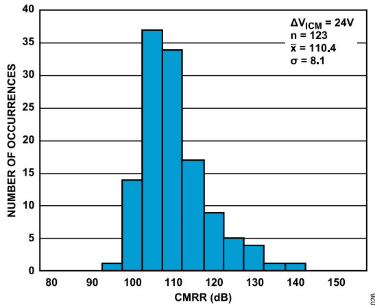
Figure 21. DC CMRR Distribution, V_{ICM} Full Range of \pm 12\text{ V} = \Delta V_{ICM} of 24 V, AFE\_GAIN = 5.2\text{ V/V} (Gain 4 Mode)
