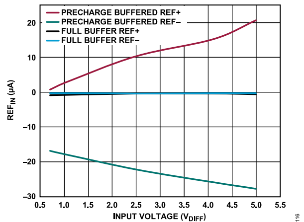
Figure 112. Reference Input Current (REF IN ) vs. Input Voltage, Precharge Buffered REF+ and REF-, and Full Buffer REF+ and REF-
