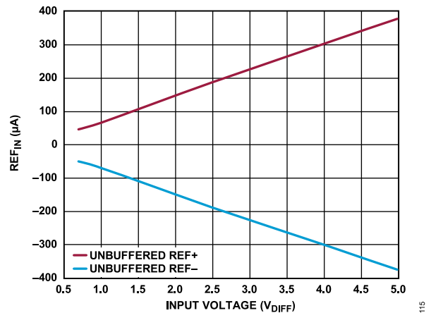
Figure 111. Reference Input Current (REF IN ) vs. Input Voltage, Unbuffered REF+ and REF-
