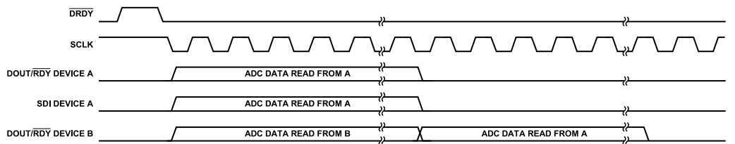
Figure 132. Data Output Format When Devices are Daisy-Chained ( \overline{\text{PIN}} Control Mode Only)
