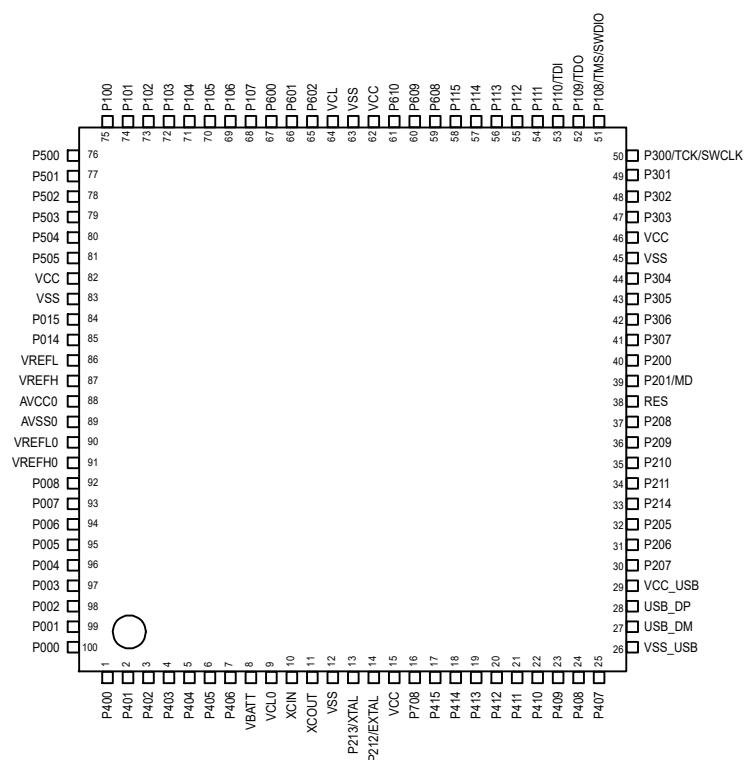
Figure 1.7 Pin assignment for LQFP 100-pin
