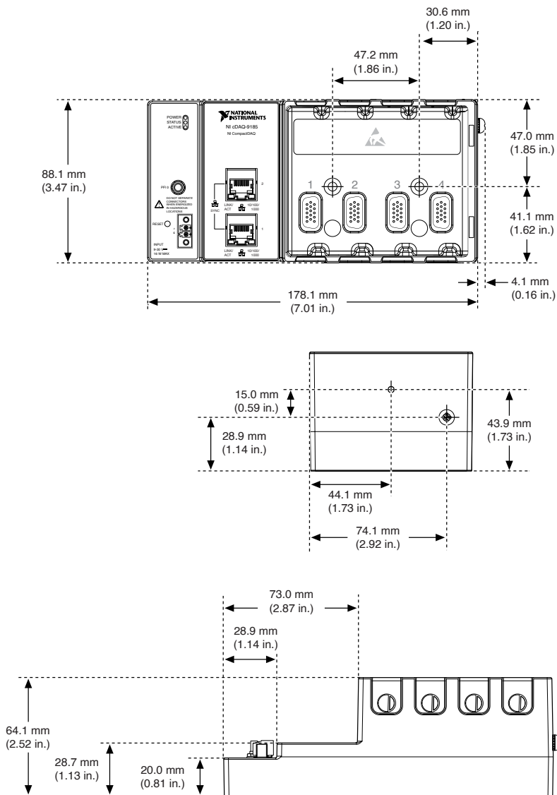
Figure 1. cDAQ-9185 Dimensions
