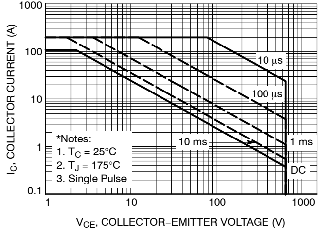
Figure 8. SOA Characteristics
