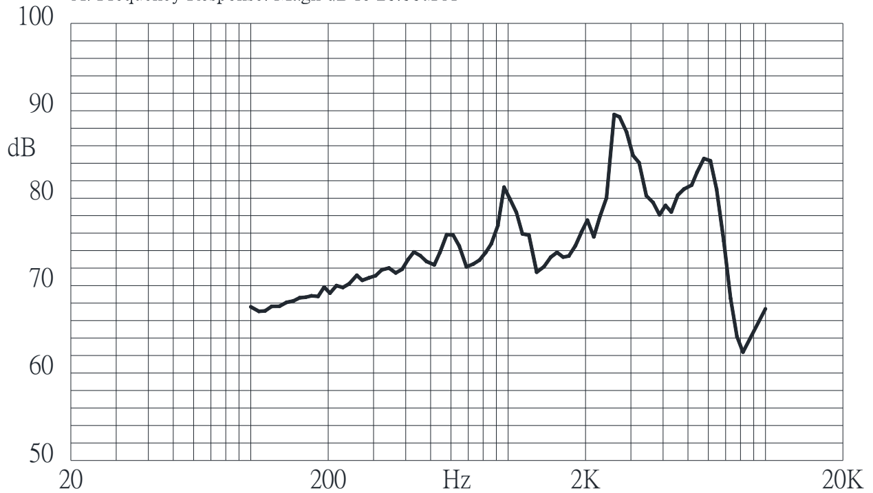
A: Frequency Response. Magn dB re 20.00uPA
