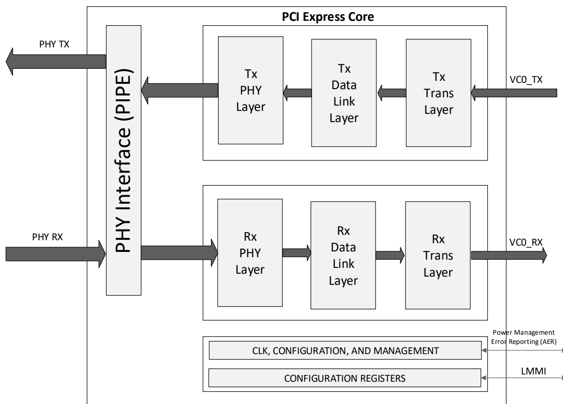
Figure 2.33. PCIe Core
