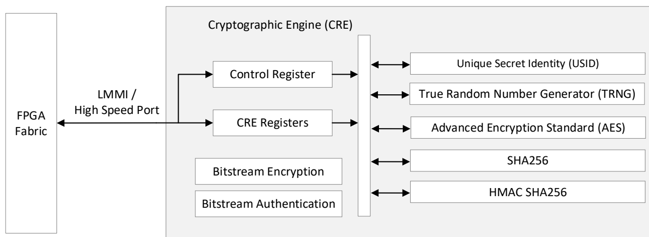
Figure 2.35. Cryptographic Engine Block Diagram
