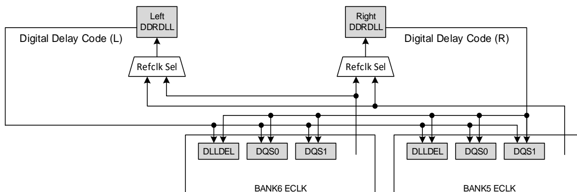
Figure 2.15. DDRDLL Architecture for MachXO5-NX-25 Devices
