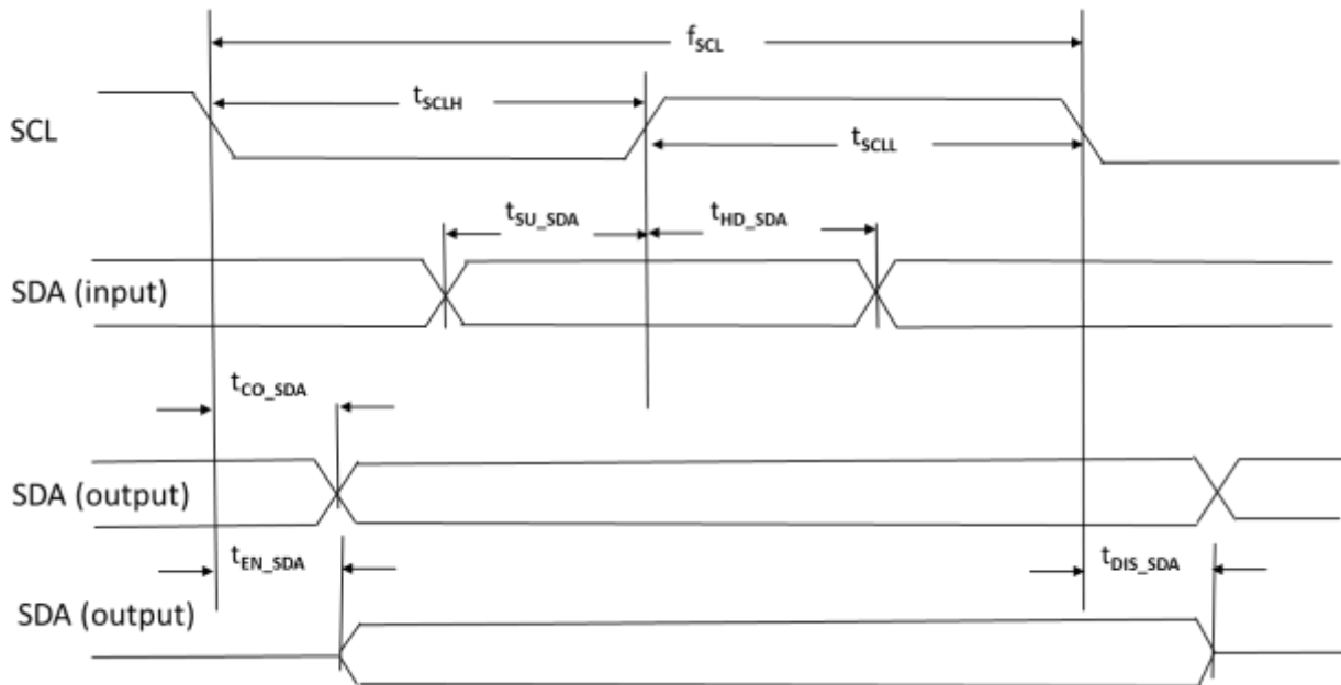
Figure 4.17. I²C / I3C Configuration Timing
