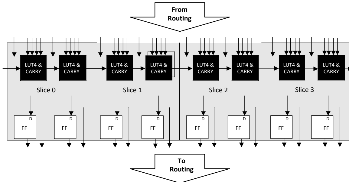
Figure 2.4. PFU Diagram
