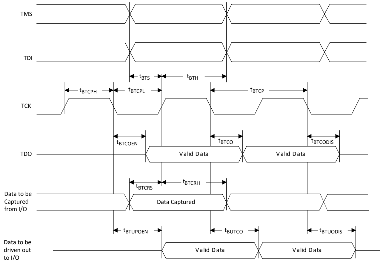
Figure 4.19. JTAG Port Timing Waveforms
