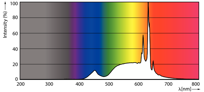
Spectral Power Distribution Colour - CoreProLEDbulb ND 4.9-40W A60 E27 927 UK
