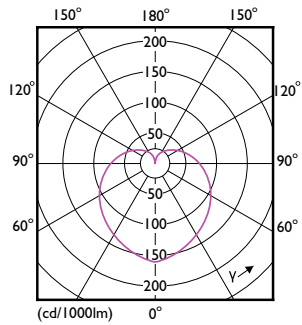
Light Distribution Diagram - CorePro LEDbulb ND 4.9-40W A60 E27 940UK
