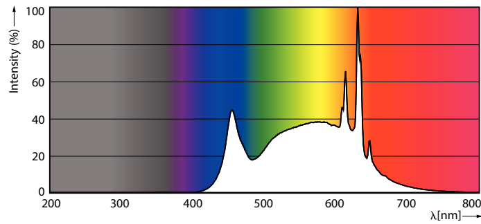
Spectral Power Distribution Colour - CorePro LEDbulb ND 4.9-40W A60 E27 940UK
