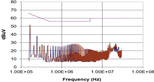
MGJ2D121805BSC (Quasi-Peak)
