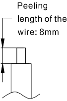
26-10AWG wires
