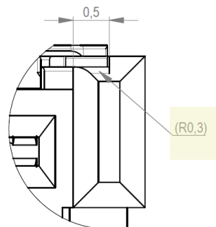
Detail X M 20:1 / scale 20:1
