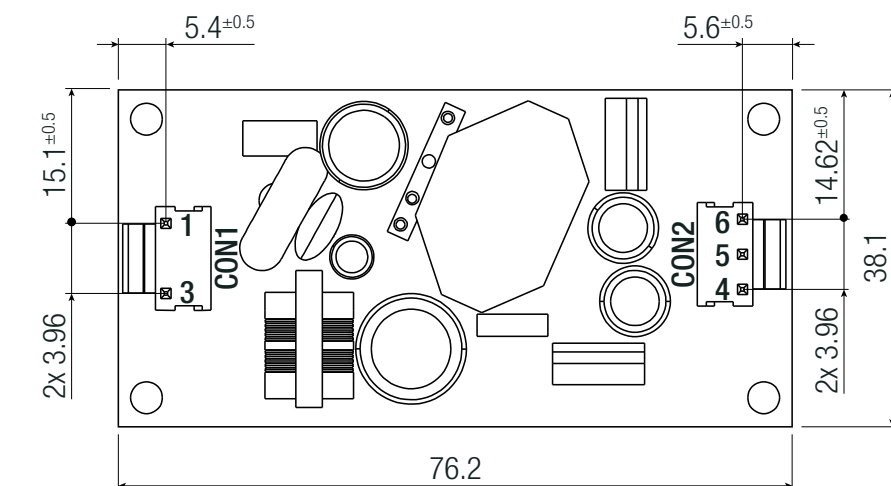
Dimension Drawing Open Frame "OF" DUAL Output (mm)
