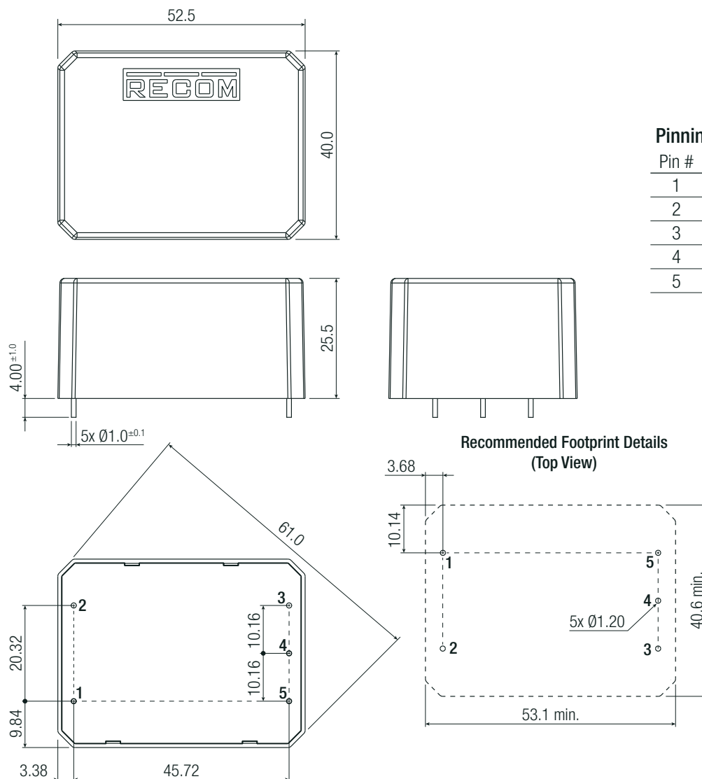
Dimension Drawing "THT printmount" version SINGLE and DUAL Output (mm)
