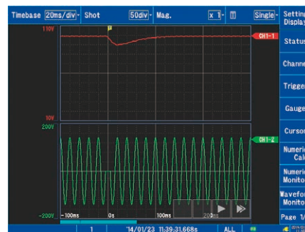
● Example of recording the instantaneous waveform and RMS level waveform during a momentary outage of an AC power supply (using the MR8905)
