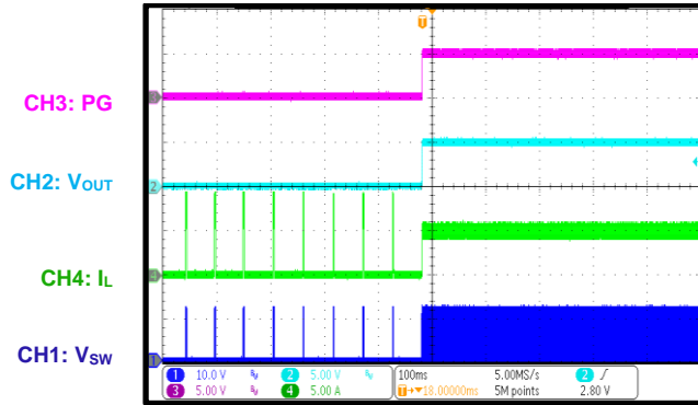
SCP Recovery I_{OUT} = 5A
