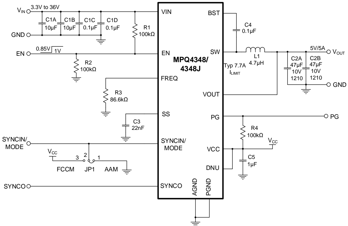
Figure 10: Typical Application Circuit (V OUT = 5V, f sw = 410kHz)
