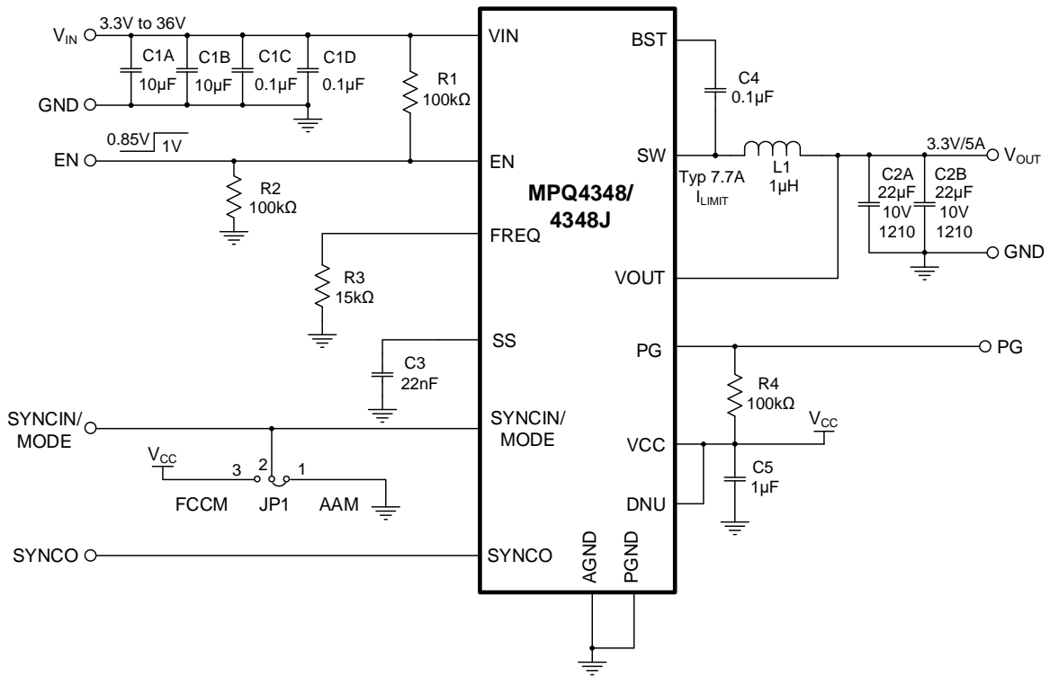
Figure 11: Typical Application Circuit (V OUT = 3.3V, f sw = 2.2MHz)
