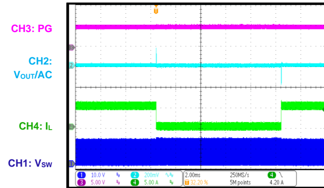
Load Transient I_{OUT} = 0A to 5A , 1.6A/\mu s slew rate
