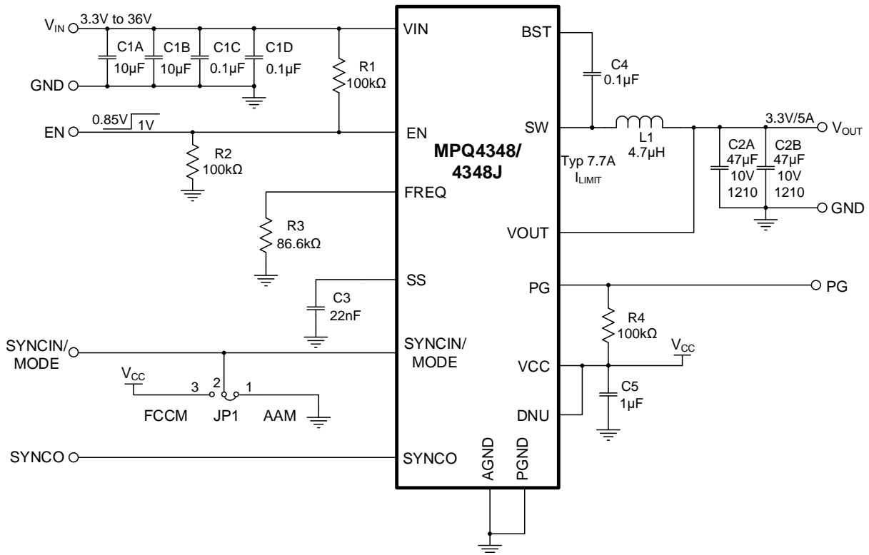
Figure 12: Typical Application Circuit (V OUT = 3.3V, f sw = 410kHz)
