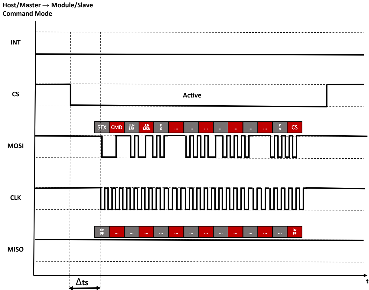
Figure 9: SPI master to slave communication, example SPI_INT "active high"
