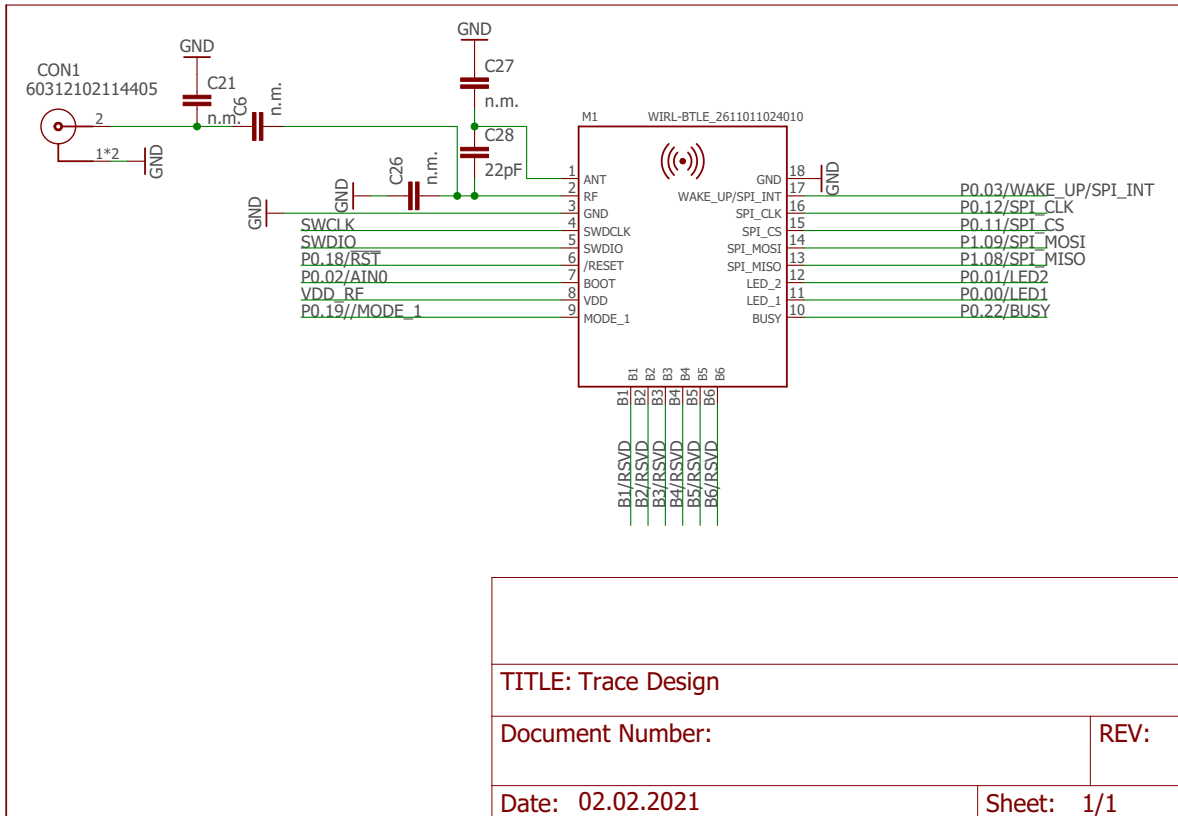
Figure 31: Trace design: Schematic
