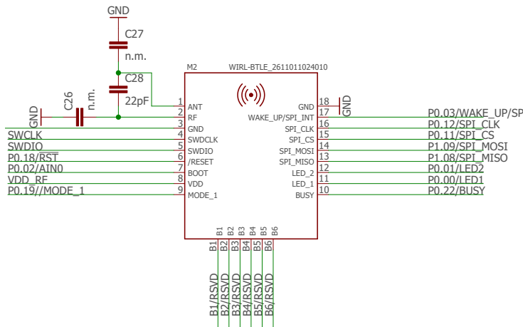
Figure 32: On-board PCB antenna
