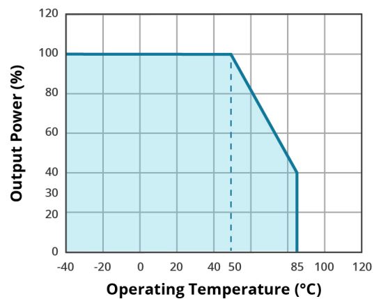
TEMPERATURE DERATING CURVE -9, -12 V output (Natural convection)
