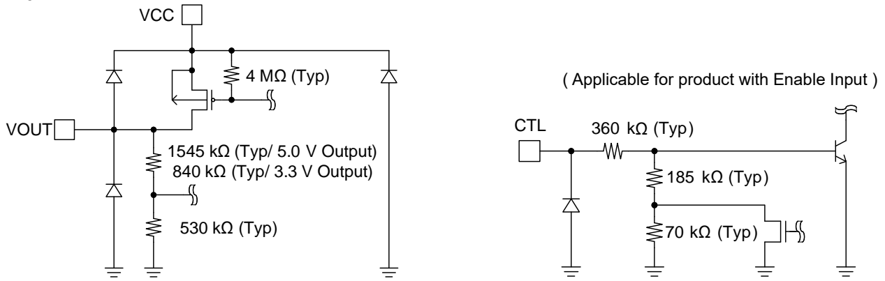
Figure 55. Input / Output Equivalence Circuit
