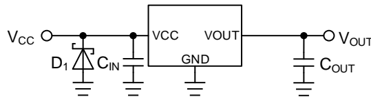
Figure 44. Surges Lower than -0.3\text{ V} is Applied to the Input
