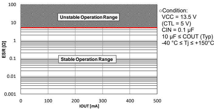
Figure 40. ESR vs IOU
