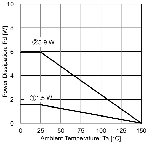
Figure 53. Package Data (TO263-5 / TO263-3)
