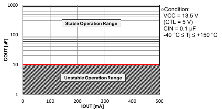
Figure 41. COU vs IOU
