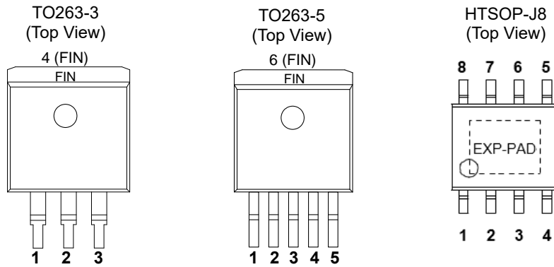
Figure 3. Pin Configurations
