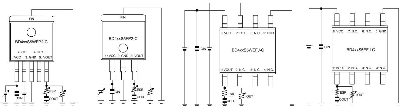
Figure 42. Measurement Setups for ESR Reference Data (about Output Pin Capacitor)
